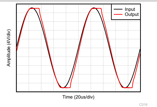
Figure 5-30. No Phase Reversal V_{IN} = \pm 20\text{ V} ; V_S = V_{OUT} = \pm 17\text{ V}
