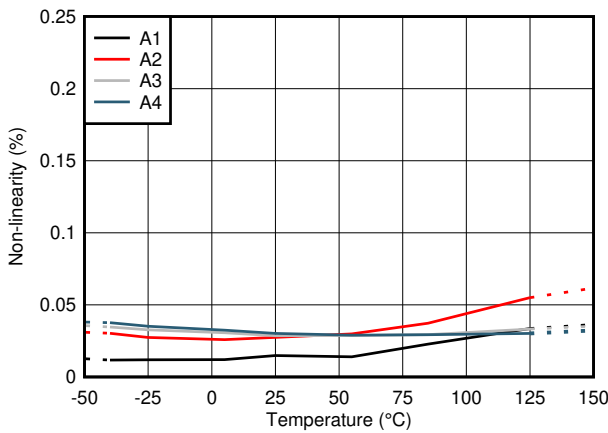
Figure 7-3. Non-Linearity vs. Temperature
