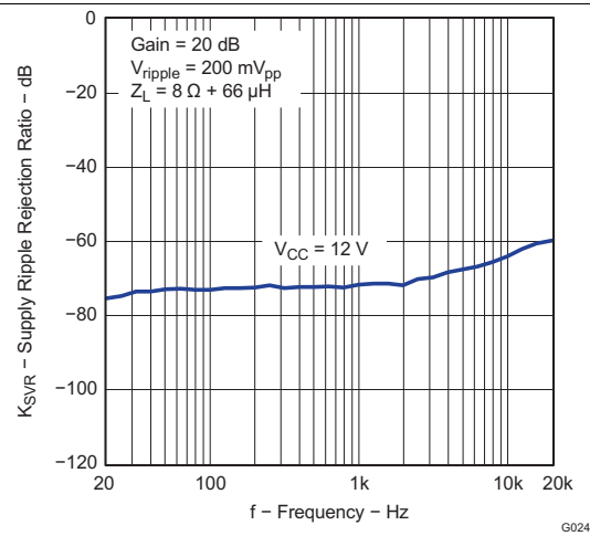
Figure 28. Supply Ripple Rejection Ratio vs Frequency (BTL)
