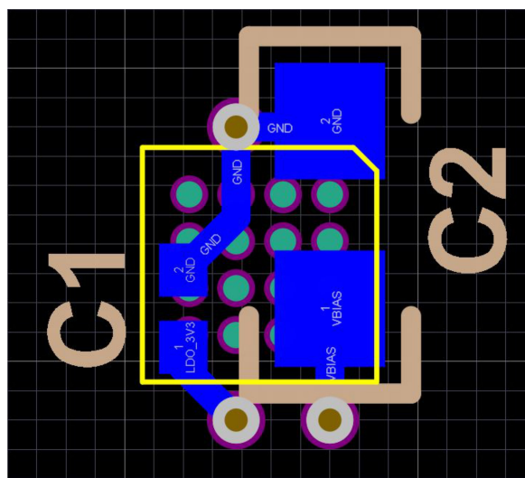
Figure 11-2. TPD4S311 Bottom Layer Routing
