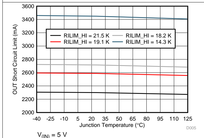
Figure 5. OUT Short-Circuit Current Limit vs Temperature I
