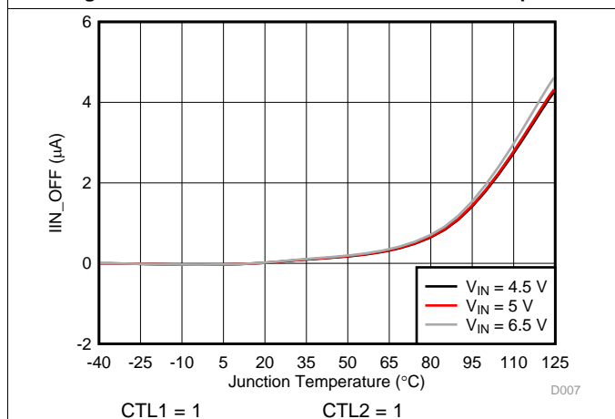
Figure 7. Disabled IN Supply Current vs Temperature
