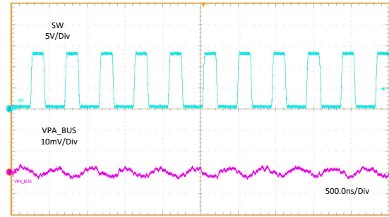
Figure 11-15. No Load Output Ripple
