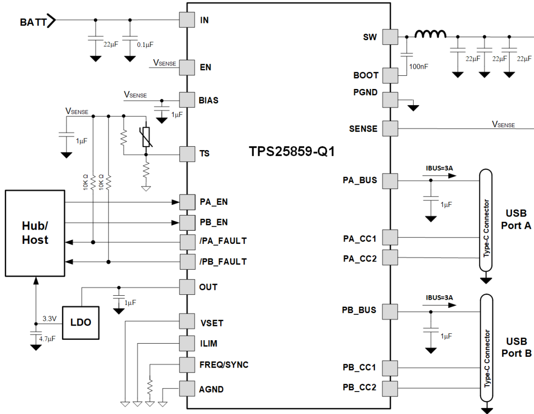
Figure 11-2. TPS25859-Q1 Typical Application Circuit for 400-kHz f_{sw}
