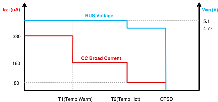
Figure 10-11. TPS25858-Q1 Behavior When Trigger Temp Warm and Hot Threshold
