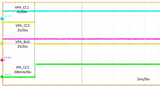
Figure 11-27. PA_CC2 Hot Short to GND
