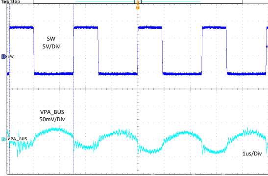
VSET = GND I_{PA\_BUS} = 0\text{ A} I_{PB\_BUS} = 0\text{ A} f_{SW} = 400\text{ kHz} Figure 11-15. No Load Output Ripple
