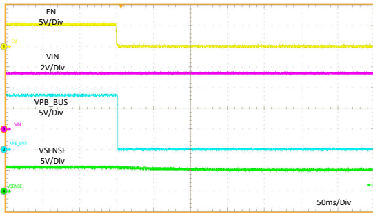
EN = 5\text{ V to }0\text{ V} PB\_CC1 = R_d I_{PB\_BUS} = 3\text{ A} Figure 11-19. Shutdown Relate to EN
