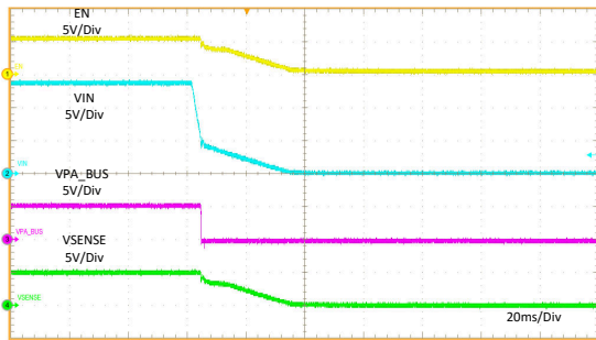
VIN = 13.5\text{ V to }0\text{ V} PA\_CC1 = R_d I_{PA\_BUS} = 3\text{ A} Figure 11-17. Shutdown Relate to VIN
