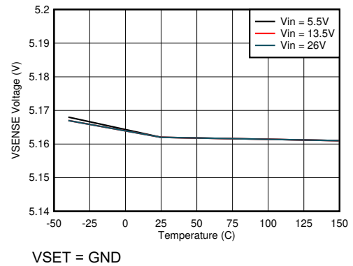
Figure 8-4. V_{SENSE} Voltage vs Junction Temperature
