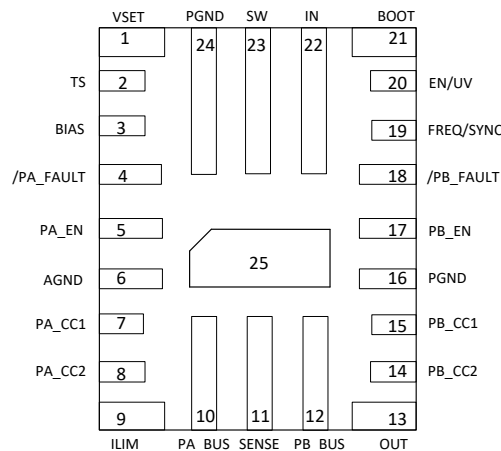
Figure 7-2. TPS25859-Q1 RPQ Package 25-Pin (QFN) Top View
