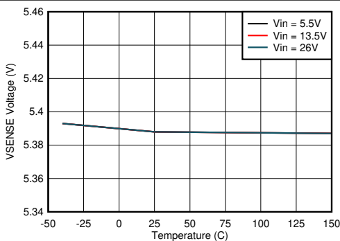
Figure 8-5. V_{SENSE} Voltage vs Junction Temperature
