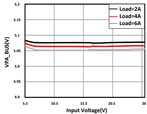
Figure 11-12. Dropout Characteristic
