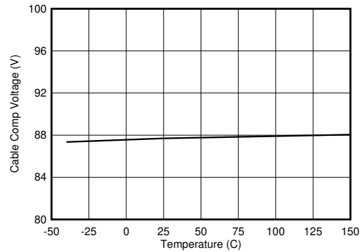
Figure 8-16. Cable Compensation Voltage vs Junction Temperature
