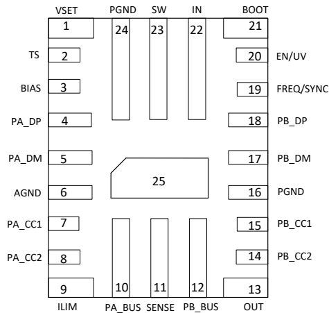
Figure 7-1. TPS25858-Q1 RPQ Package 25-Pin (QFN) Top View
