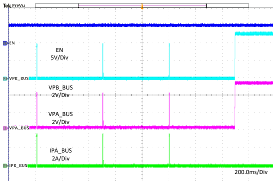
Figure 11-25. 1-Ω Load Recovery
