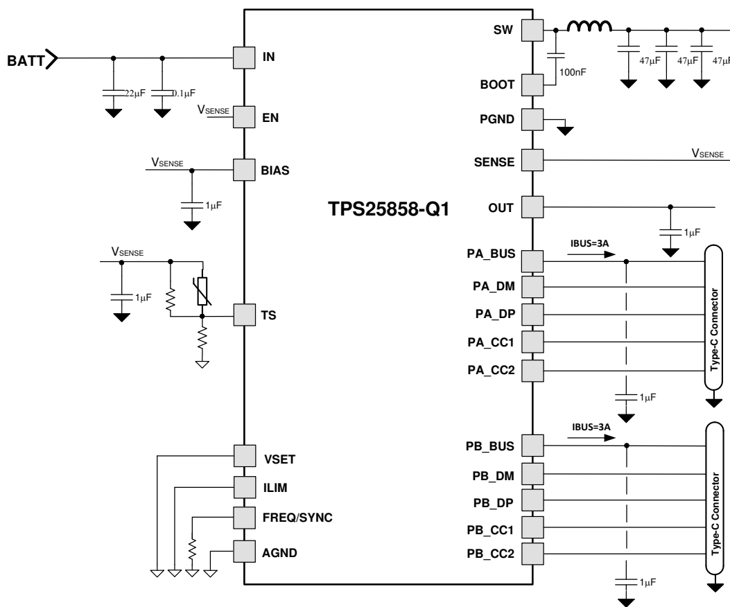
Figure 11-1. TPS25858-Q1 Typical Application Circuit for 400-kHz f_{sw}
