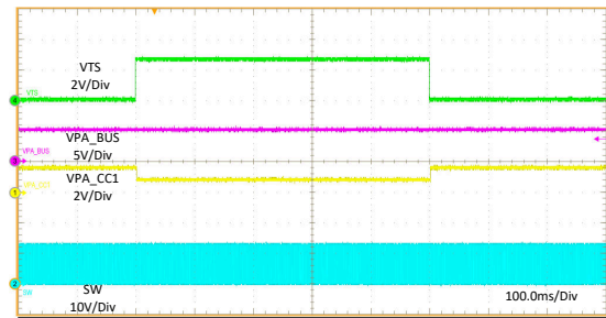
Figure 11-28. OUT short to 5.1- \Omega Load
