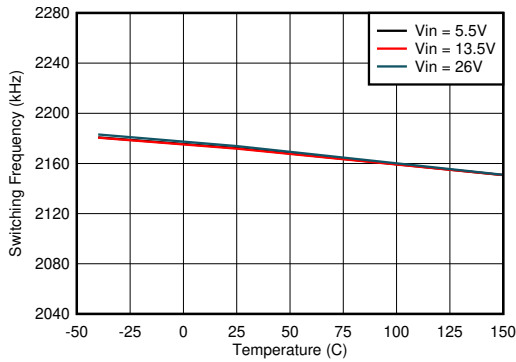
Figure 8-21. Switching Frequency vs Junction Temperature
