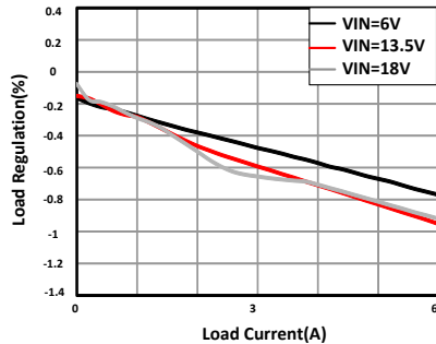
Figure 11-5. Load Regulation
