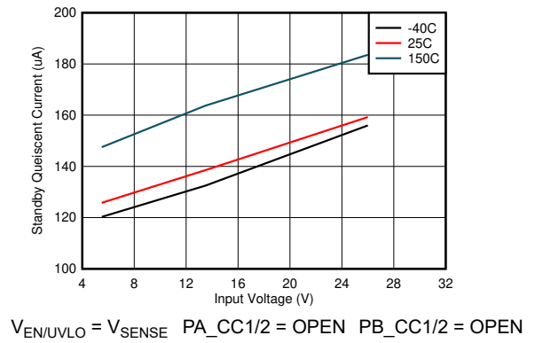
Figure 8-2. Standby Quiescent Current
