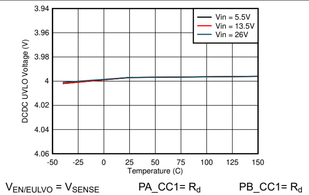
Figure 8-6. DCDC UVLO Threshold
