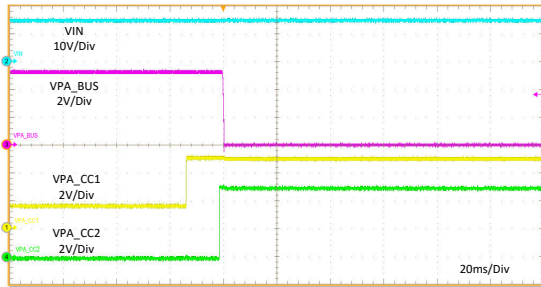
PA_CC1 = R d to Open PA_CC2 = Open I PA_BUS = 3 A Open
