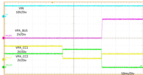
PA\_CC1 = \text{Open to } R_d PA\_CC2 = \text{Open} I_{PA\_BUS} = 3\text{ A} Figure 11-20. Rd Assert
