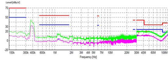
Figure 11-4. 400-kHz EMI Results (Without CM Filter)
