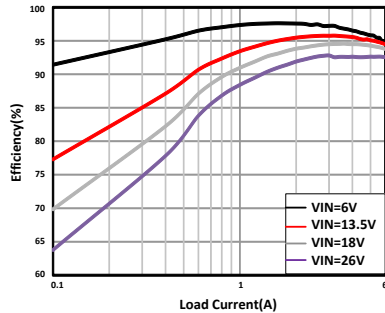
Figure 11-3. Buck Only Efficiency
