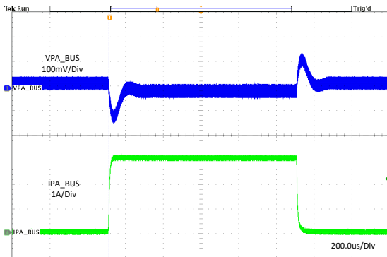
Figure 11-5. Load Regulation
