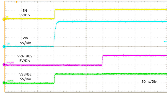
VIN = 0\text{ V to }13.5\text{ V} PA\_CC1 = R_d I_{PA\_BUS} = 3\text{ A} Figure 11-16. Startup Relate to VIN
