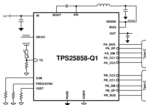
Simplified Schematic: TPS25858-Q1
