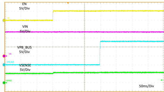
EN = 0\text{ V to }5\text{ V} PB\_CC1 = R_d I_{PB\_BUS} = 3\text{ A} Figure 11-18. Startup Relate to EN
