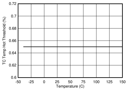
Figure 8-24. TS Temperature Hot Threshold vs Junction Temperature
