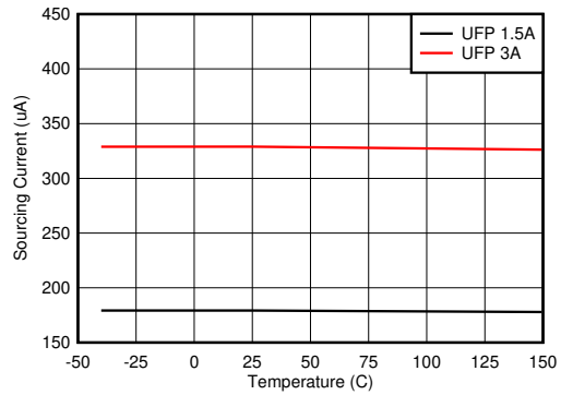
Figure 8-22. CC Sourcing Current vs Junction Temperature
