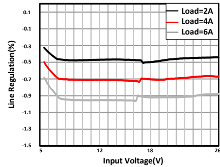
Figure 11-6. Line Regulation
