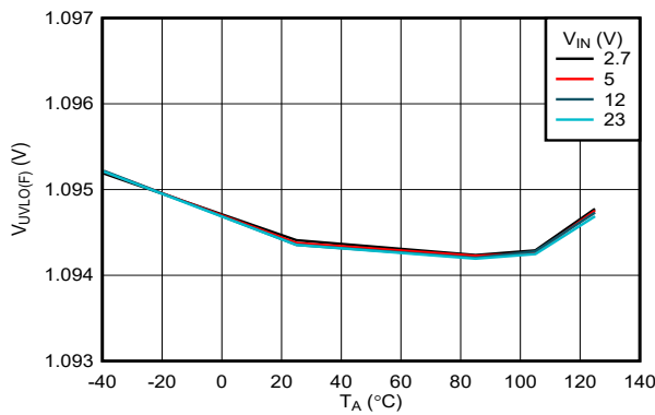
Figure 7-10. EN/UVLO Falling Threshold vs Temperature
