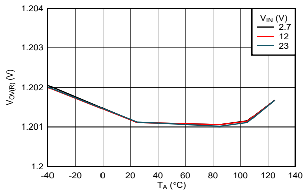
Figure 7-12. OVLO Rising Threshold vs Temperature
