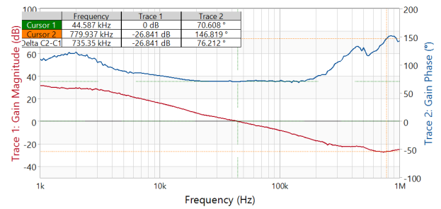
Figure 8-25. Closed loop bode plot channel B
