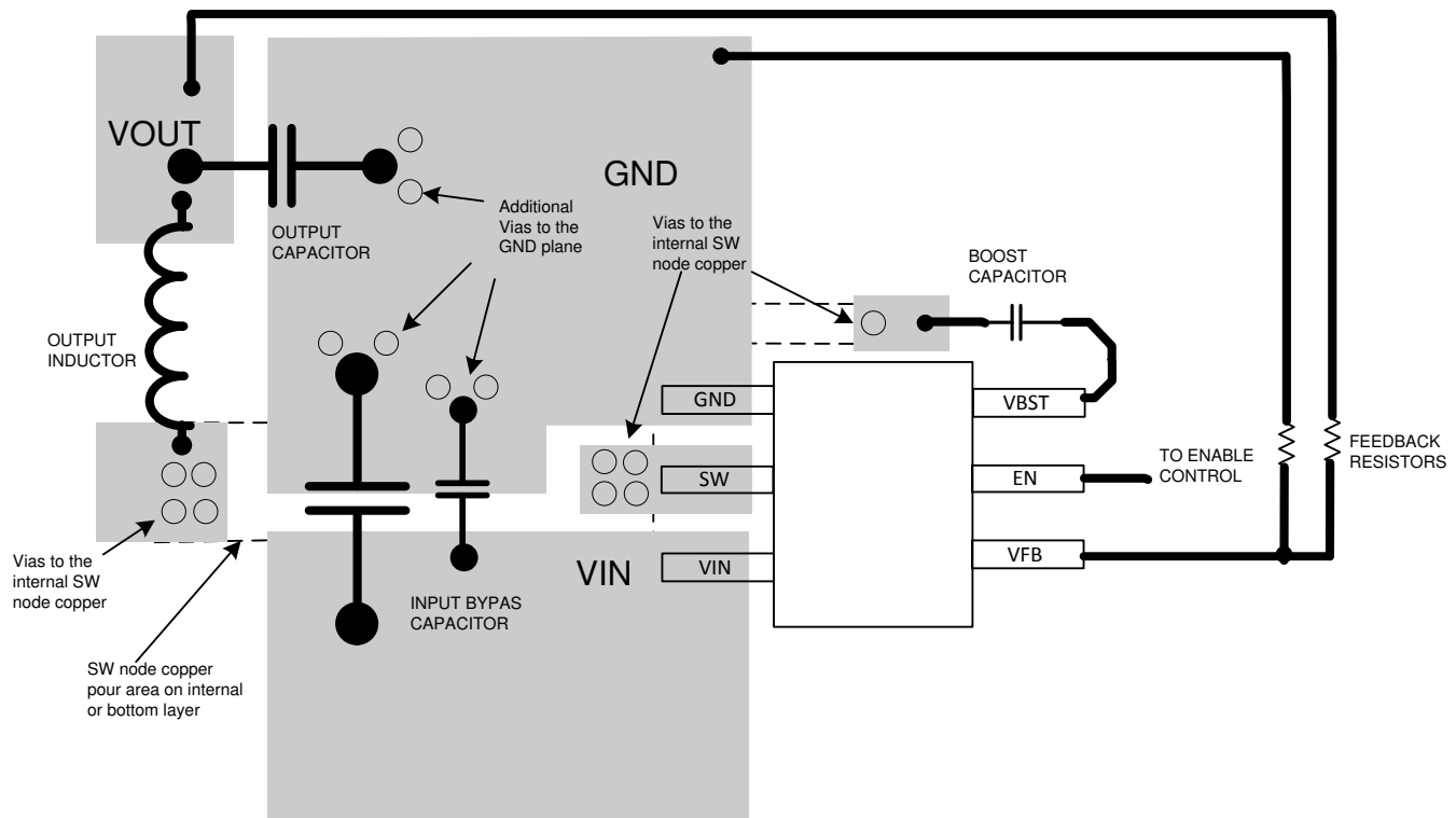
Figure 10-1. Board Layout
