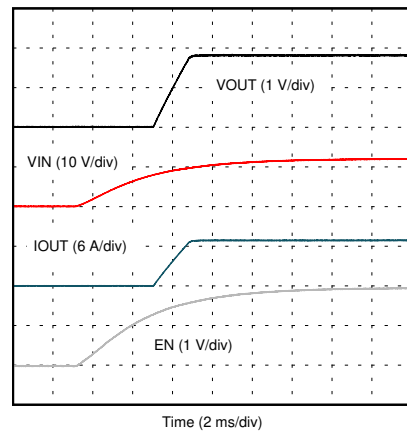
Figure 7-17. EN Start-Up – DCM
