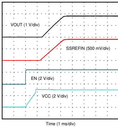
Figure 7-16. EN Start-Up
