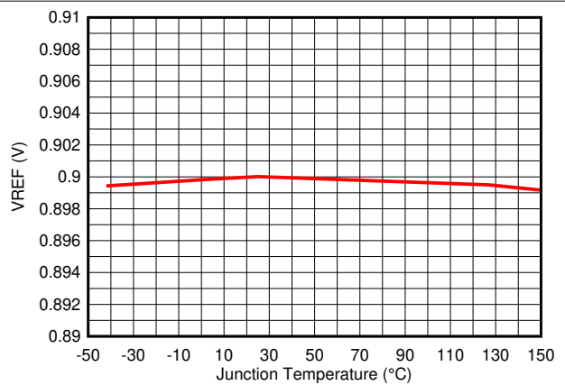
Figure 5-6. Vref
