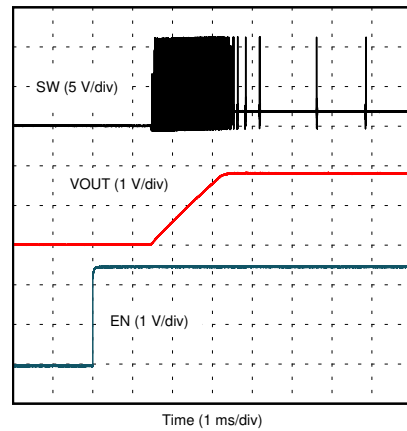
Figure 7-15. EN Start-Up
