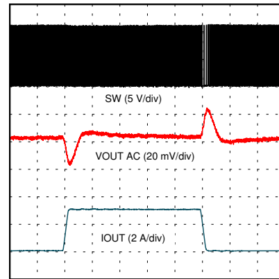
Time (20 \mu s/div) V_{IN} = 12 \text{ V} 0.1 A to 3.1 A step 1 A/ \mu sec MODE = FCCM
