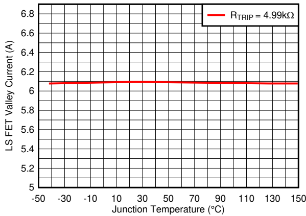
Figure 5-3. Overcurrent Limit
