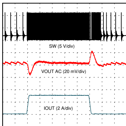
Time (20 \mu s/div) V_{IN} = 12 \text{ V} 0.1 A to 3.1 A step 1 A/ \mu sec MODE = DCM
