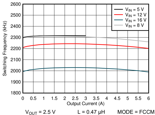
Figure 5-17. 2200-kHz Switching Frequency vs Load Current
