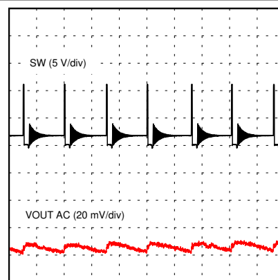
Time (4 \mu s/div) V_{IN} = 12 \text{ V} I_{LOAD} = 0.1 \text{ A} MODE = DCM
