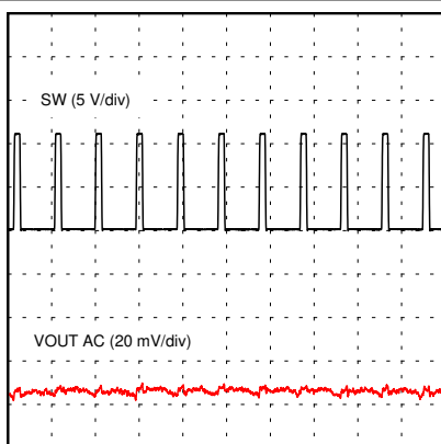
Time (1 \mu s/div) V_{IN} = 12 \text{ V} I_{LOAD} = 0.1 \text{ A} MODE = FCCM
