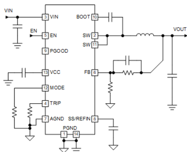
Simplified Schematic
