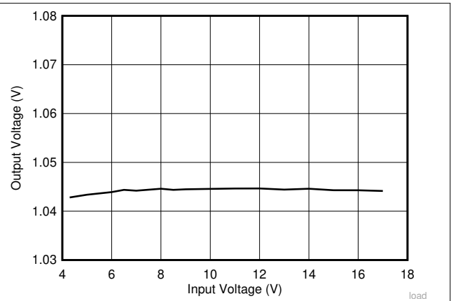
Figure 9-3. Load Regulation with Different Input Voltage
