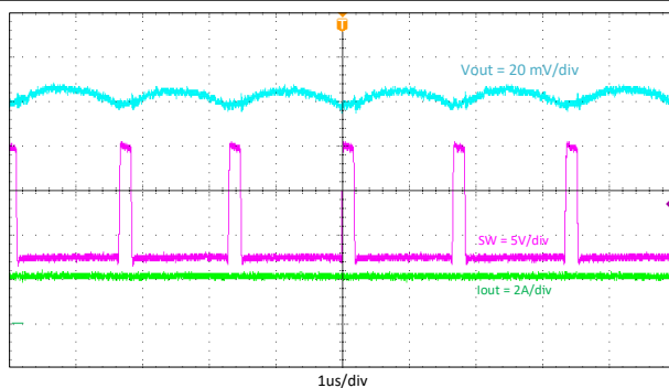
Figure 9-6. Output Voltage Ripple, I_{out} = 2\text{ A}
