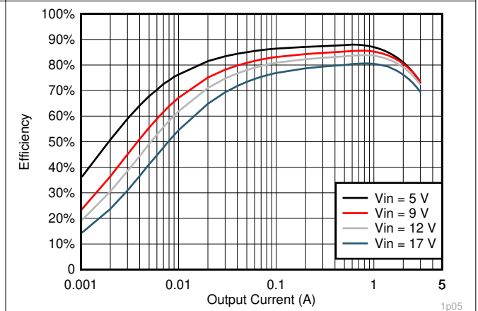
Figure 7-10. V_{OUT} = 1.05 V Efficiency, L = 1.2 \mu\text{H}
