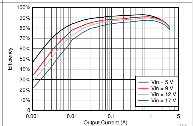
Figure 7-12. V_{OUT} = 1.8 V Efficiency, L = 2.2 \mu\text{H}
