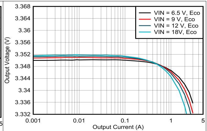
Figure 8-3. Load Regulation
