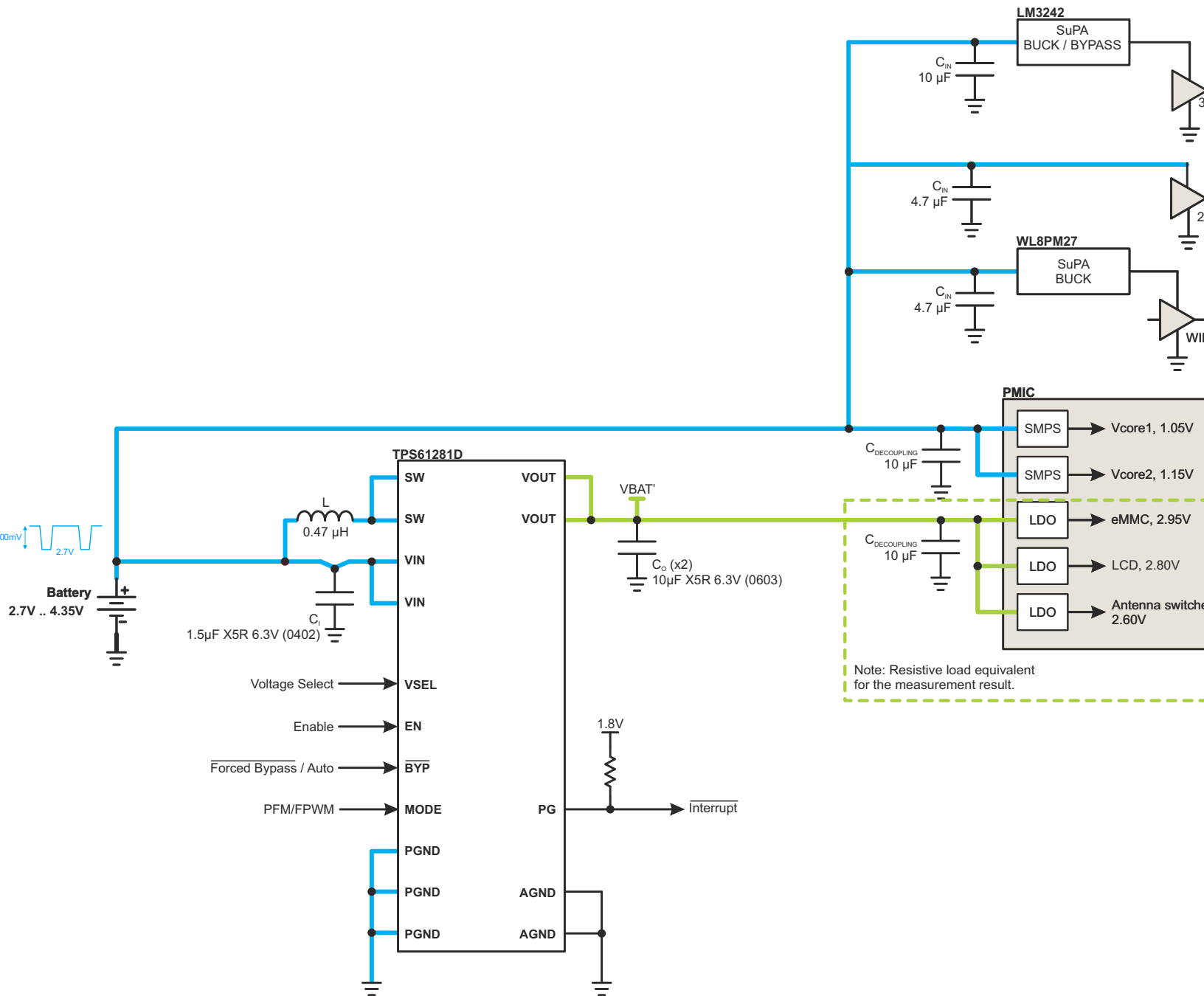
Figure 10-1. TPS61281D Application Circuit with 150mA Output Current
