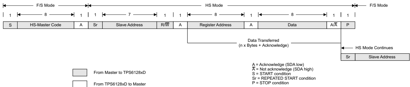
Figure 9-12. Data Transfer Format in H/S-Mode
