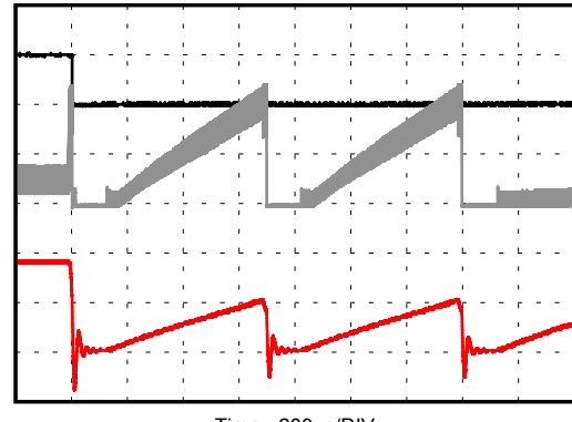
Figure 9-34. HICCUP Short Circuit Protection
