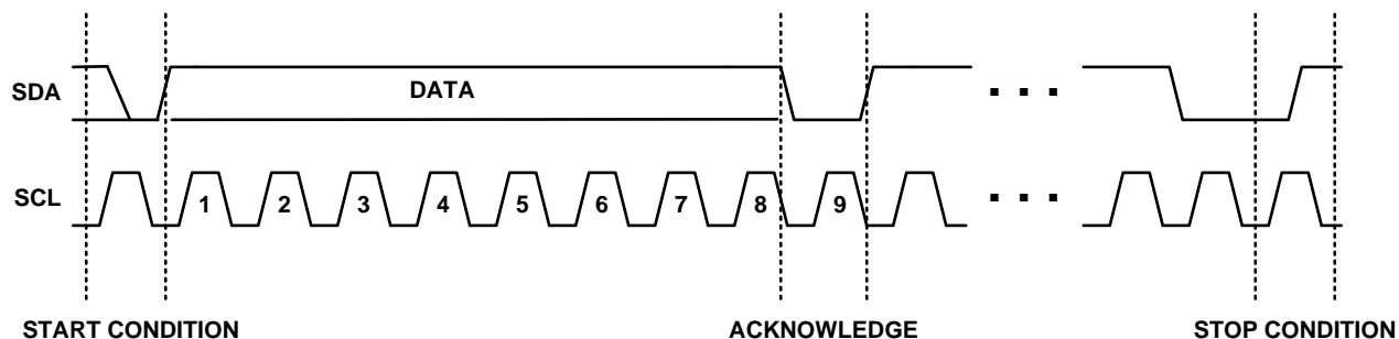
Figure 15. I 2 C Start / Stop / Acknowledge Protocol
