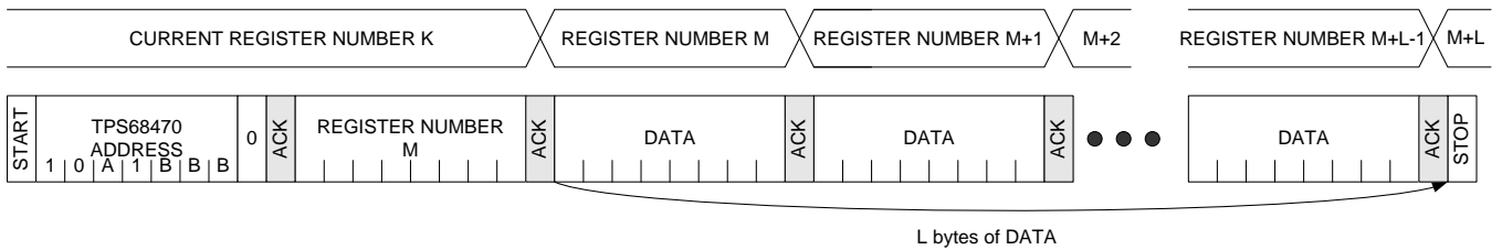
Figure 12. Sequential Write
