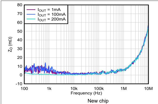
Figure 5-13. Output Impedance vs Frequency
