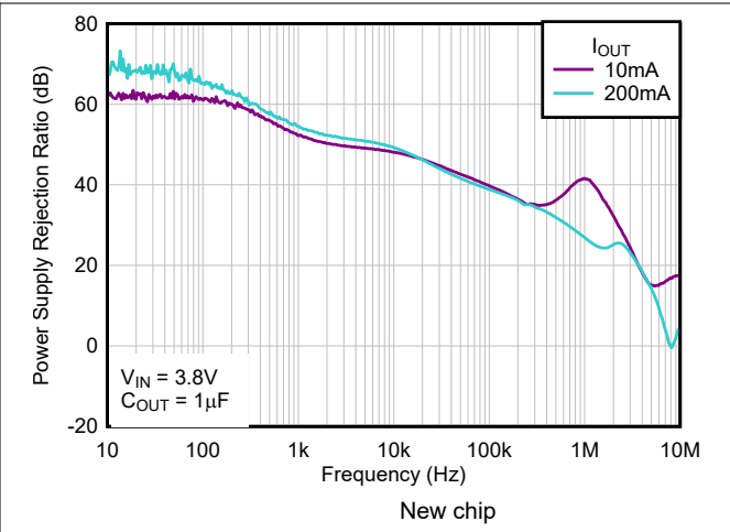
Figure 5-20. TPS793 Ripple Rejection vs Frequency
