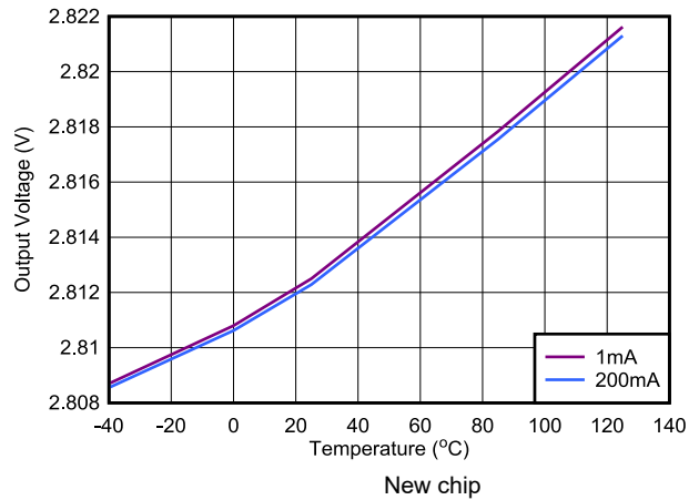
Figure 5-4. TPS793 Output Voltage vs Junction Temperature
