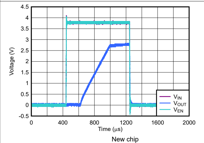
Figure 5-22. TPS793 Output Voltage, Enable Voltage vs Time (Start-Up)
