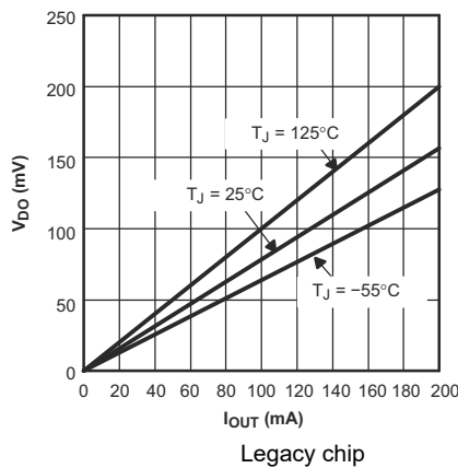
Figure 5-29. Dropout Voltage vs Output Current
