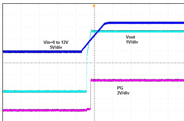
Figure 27. Power Up (5 V), 20 ms/div, I L = 20 mA
