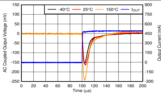
V_{OUT} = 5\text{ V} , I_{OUT} = 0\text{ mA} to 500\text{ mA} , slew rate = 1\text{ A}/\mu\text{s} , C_{OUT} = 10\ \mu\text{F}
