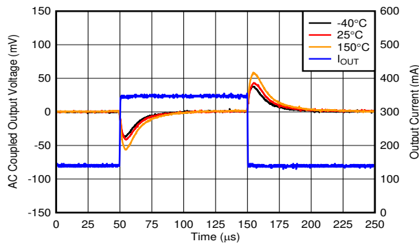
V_{OUT} = 5\text{ V} , I_{OUT} = 150\text{ mA} to 350\text{ mA} , slew rate = 0.1\text{ A}/\mu\text{s} , C_{OUT} = 10\ \mu\text{F}
