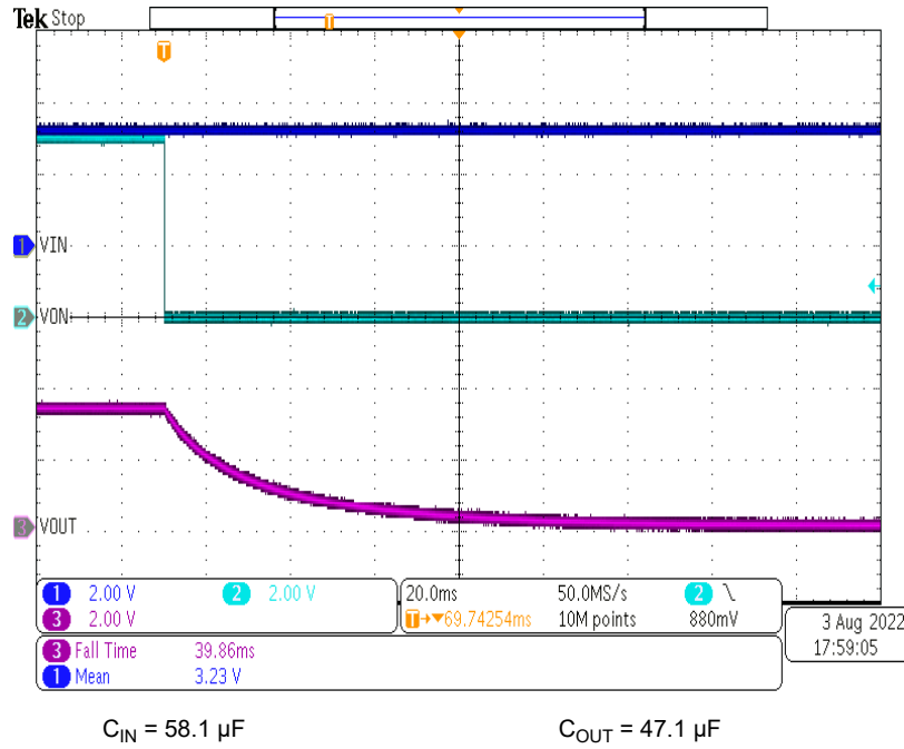
Figure 9-2. Fall Time (R QOD = 1 kΩ)
