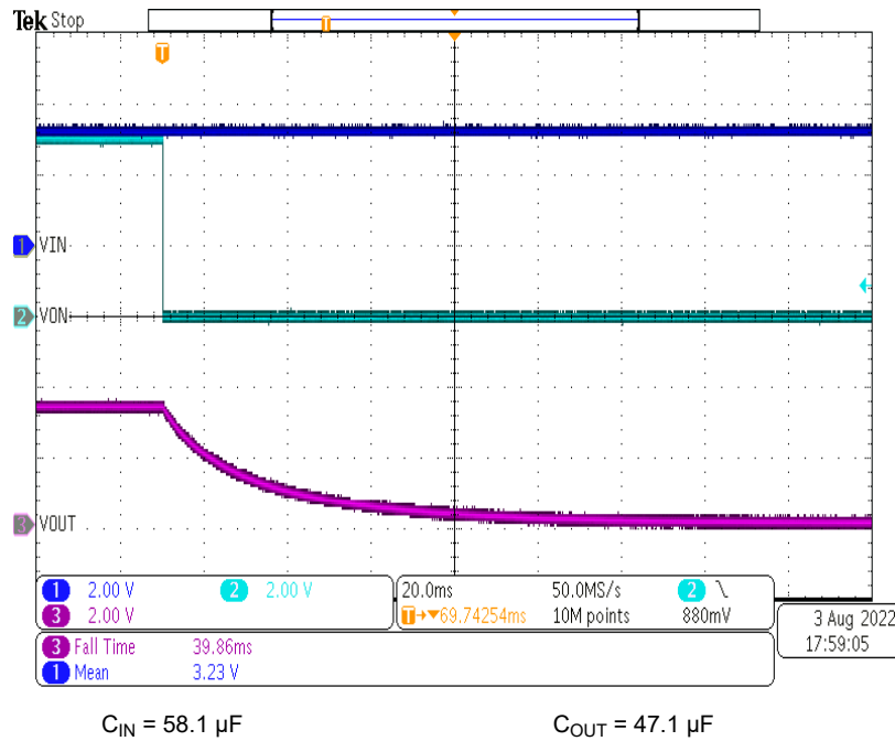
Figure 9-3. Fall Time (R QOD = 1 kΩ)
