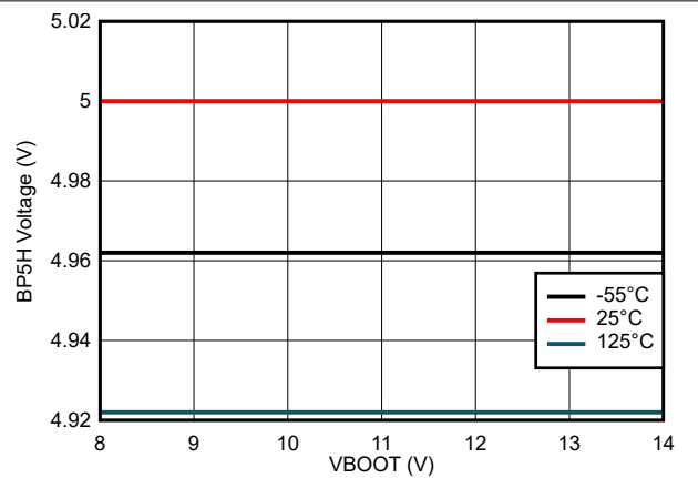
Figure 7-2. BP5H Output Voltage vs BOOT Voltage
