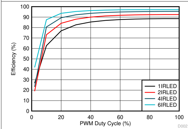
Figure 6-15. Efficiency at 1-A Output Current, 4.7- \mu\text{H} Inductor, 12-V Input Voltage
