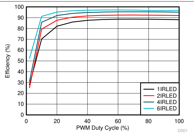
Figure 6-16. Efficiency at 1.5-A Output Current, 4.7- \mu\text{H} Inductor, 12-V Input Voltage
