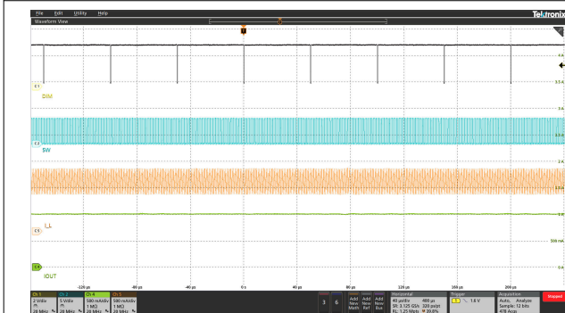
Figure 8-33. LED Analog Dimming at 1% Duty Cycle and 20 kHz
