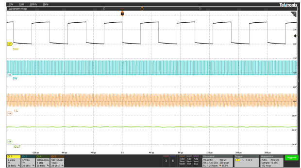
Figure 8-34. LED Analog Dimming at 50% Duty Cycle and 20 kHz
