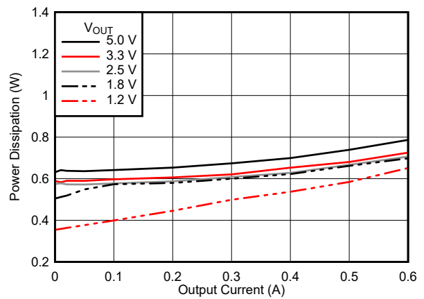
Figure 6-14. Power Dissipation
