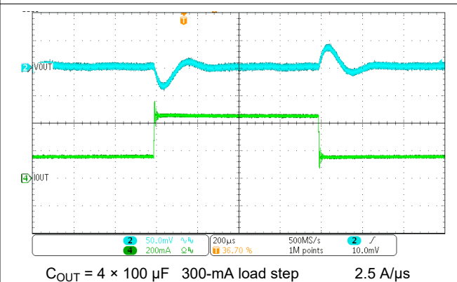
Figure 8-5. Transient Response Waveform
