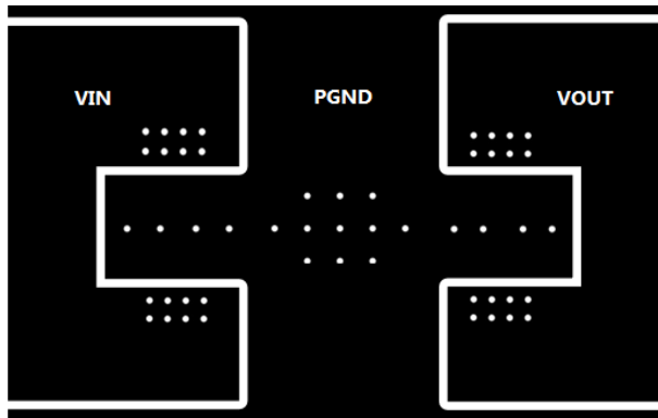
Figure 10-3. Typical Mid-Layer
