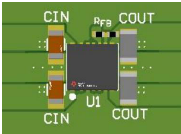
Figure 10-1. Typical Layout
