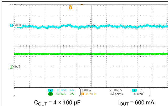
Figure 8-4. Output Ripple Waveform
