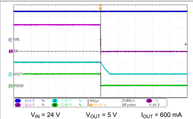
Figure 8-3. Enable Shutdown Waveforms
