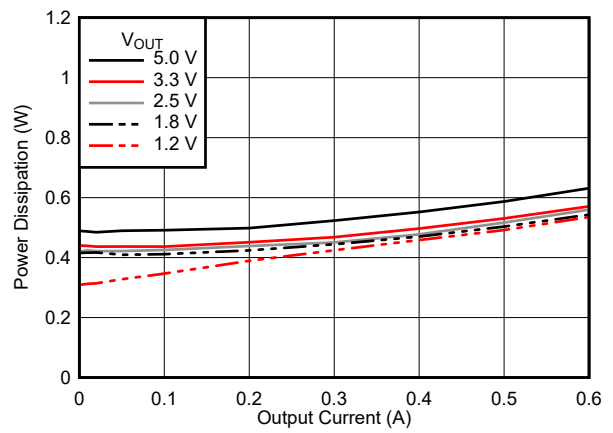
Figure 6-10. Power Dissipation
