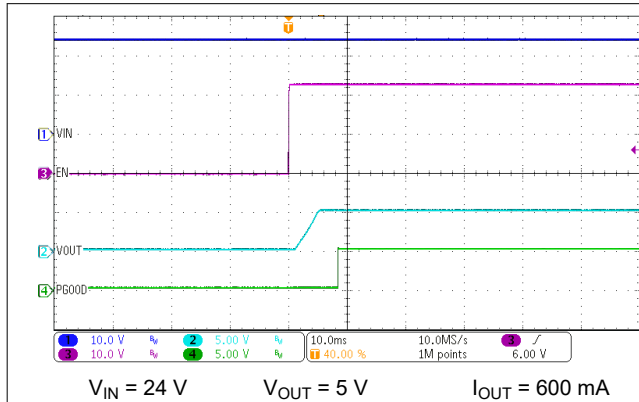
Figure 8-2. Start-Up Waveforms
