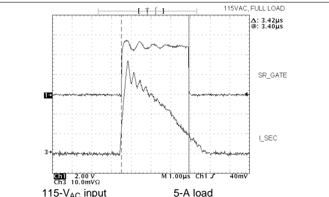
115-V AC input 5-A load Figure 27. SR MOSFET Drain Current and SR GATE Signal
