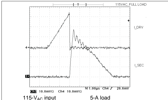
115-V AC input 5-A load Figure 26. Primary and Secondary MOSFET Currents
