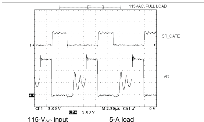
115-V AC input 5-A load Figure 28. SR MOSFET Gate and Drain Waveforms
