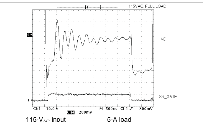
115-V AC input 5-A load Figure 29. Close-Up View of VD and SR GATE
