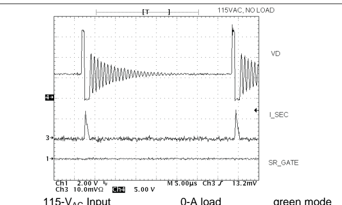
115-V AC Input 0-A load green mode Figure 31. Secondary-Side Waveforms
