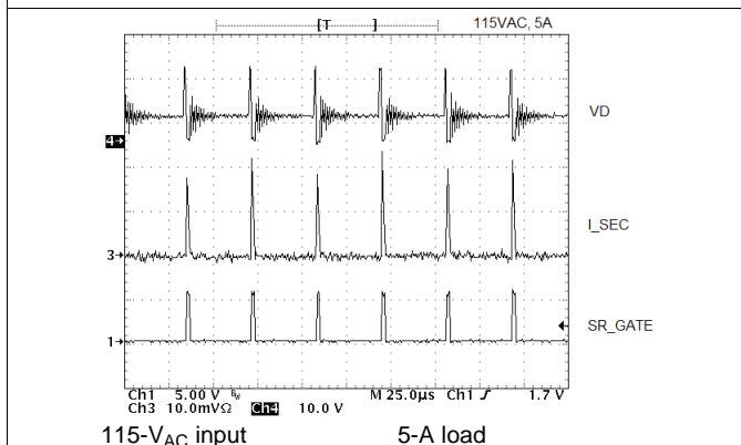
115-V AC input 5-A load Figure 30. Secondary-Side Waveforms
