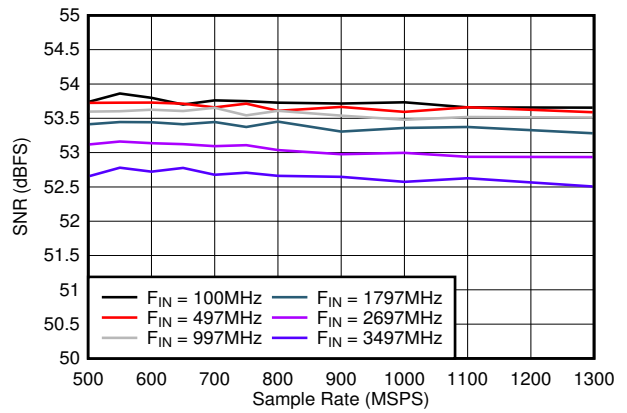
Figure 7-22. SNR vs Sample Rate
