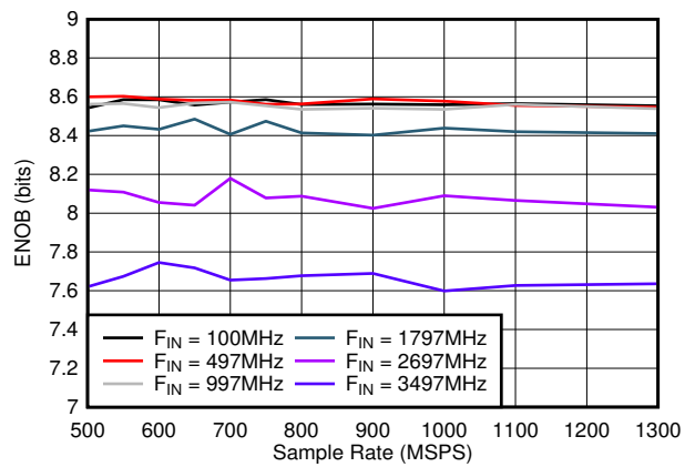
Figure 7-24. ENOB vs Sample Rate
