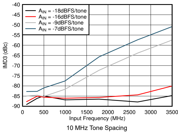
Figure 5-57. IMD3 vs Input Frequency
