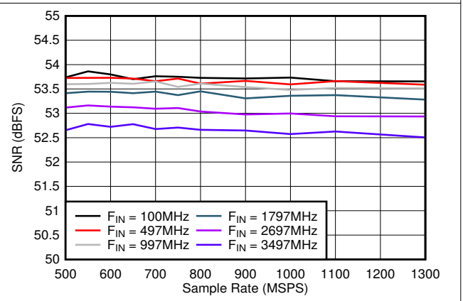
Figure 5-22. SNR vs Sample Rate
