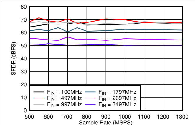
Figure 5-21. SFDR vs Sample Rate
