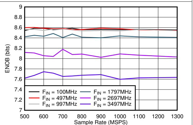
Figure 5-24. ENOB vs Sample Rate
