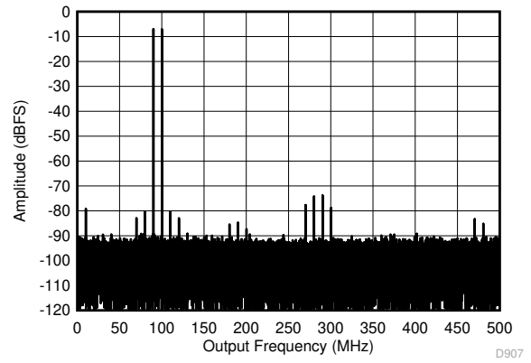
Figure 5-54. Two Tone FFT at 95.07 MHz Center
