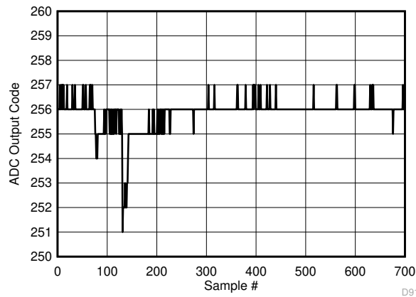
Figure 5-129. Background Calibration Core Transition (DC Signal)
