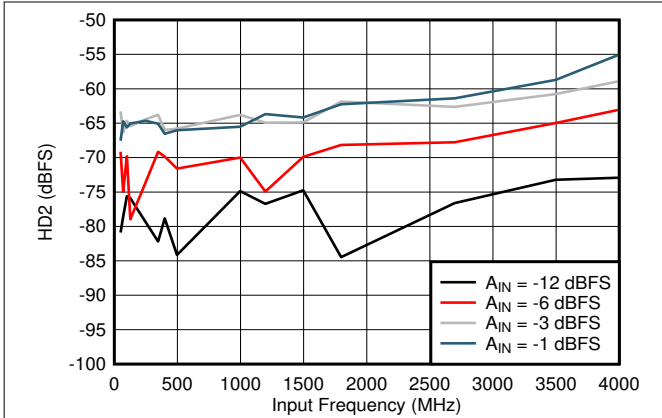
Figure 5-19. HD2 vs Input Frequency
