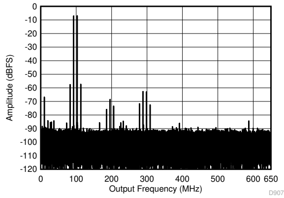
Figure 5-53. Two Tone FFT at 2698 MHz Center
