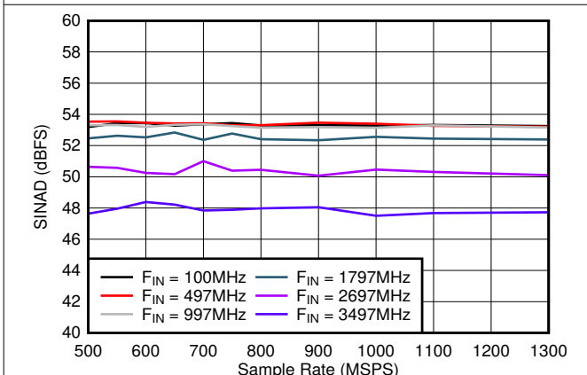
Figure 5-23. SINAD vs Sample Rate
