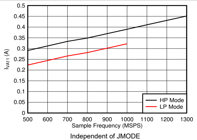
Figure 5-96. Dual Channel, I_{VA11} vs FS
