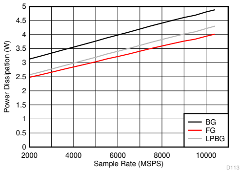
JMODE 1 Figure 5-129. DES Mode: Power Dissipation vs Sample Rate
