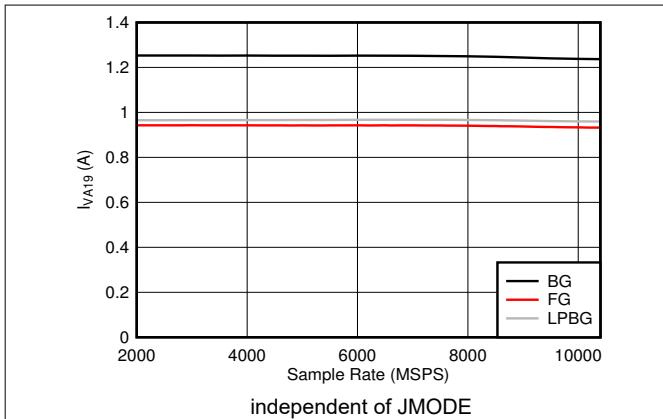
Figure 5-123. DES Mode: I_{VA19} vs Sample Rate
