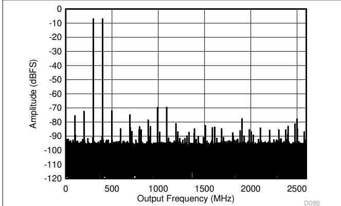
Figure 5-23. Dual Channel Mode: Two Tone FFT at 347 MHz
