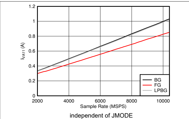
Figure 5-124. DES Mode: I_{VA11} vs Sample Rate
