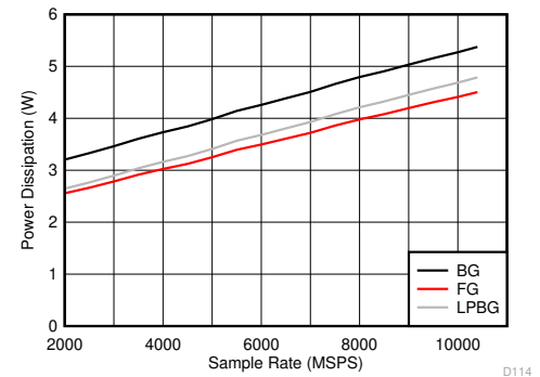
JMODE 21 Figure 5-130. DES Mode: Power Dissipation vs Sample Rate
