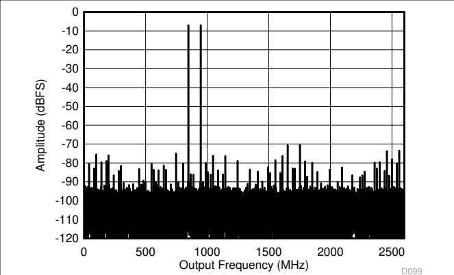
Figure 5-24. Dual Channel Mode: Two Tone FFT at 897 MHz
