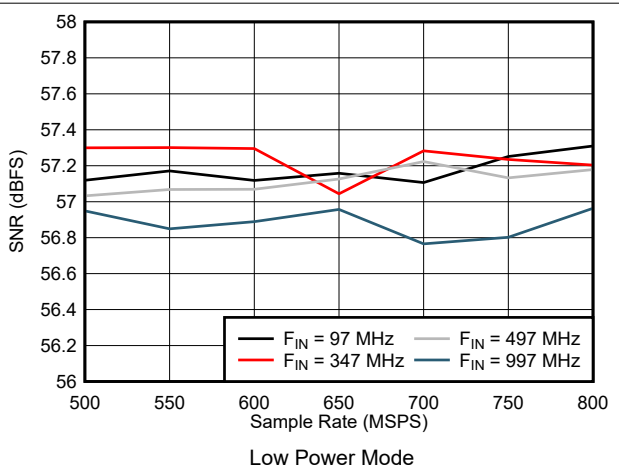
Figure 5-54. SNR vs Sample Rate in Low Power Mode
