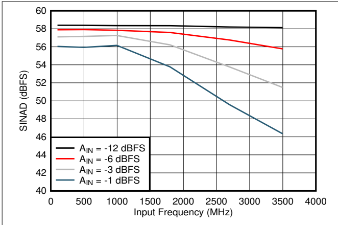
Figure 5-19. SINAD vs Input Frequency
