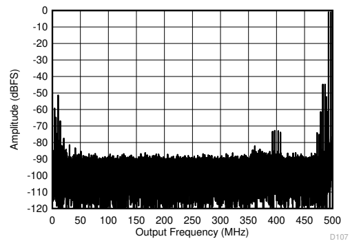
Figure 5-74. Two Tone FFT at 3498 MHz
