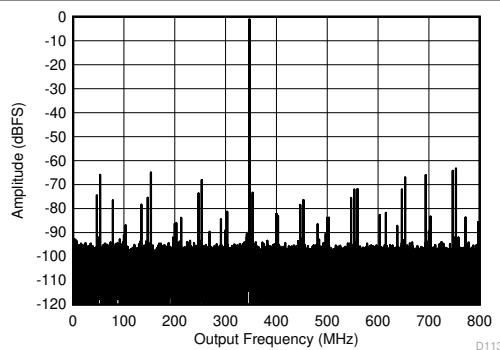
High power mode, C-PLL on, Noise suppression off Figure 5-6. Single Tone FFT at 347 MHz and -1 dBFS
