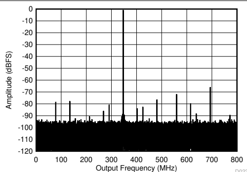
High power mode Figure 5-4. Single Tone FFT at 347 MHz and -1 dBFS
