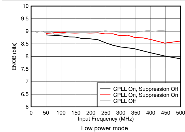
Figure 5-47. ENOB vs F_{IN} and C-PLL modes
