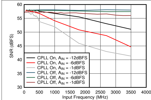
Figure 5-49. SNR vs A_{IN} and C-PLL
