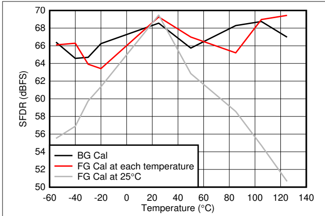
Figure 5-65. SFDR vs Temperature
