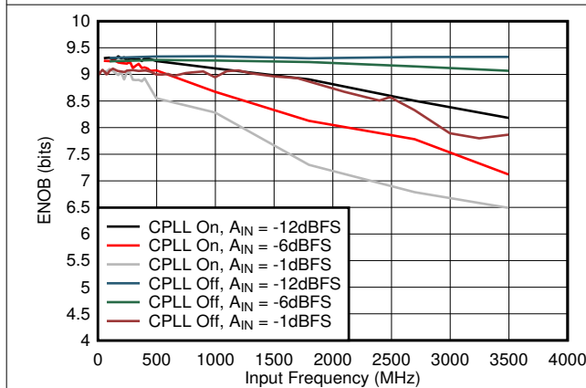
Figure 5-51. ENOB vs A_{IN} and C-PLL
