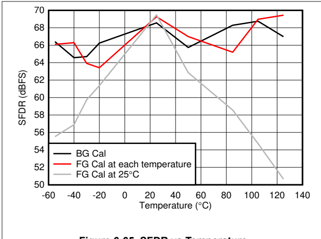
Figure 6-65. SFDR vs Temperature
