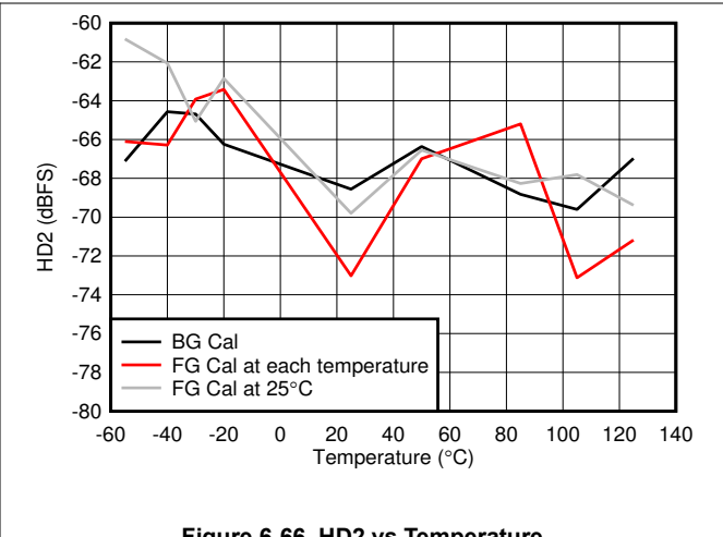
Figure 6-66. HD2 vs Temperature
