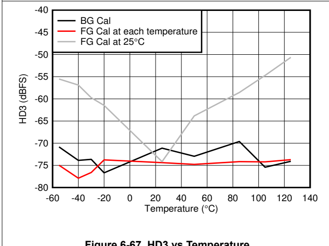
Figure 6-67. HD3 vs Temperature
