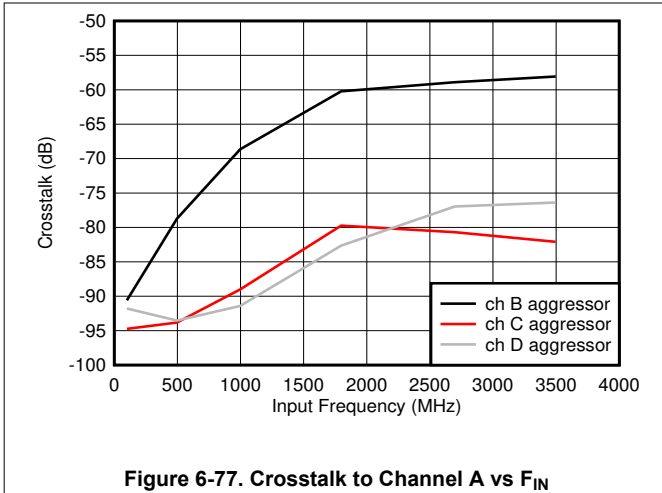
Figure 6-77. Crosstalk to Channel A vs F_{IN}
