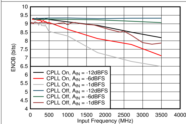
Figure 6-51. ENOB vs A_{IN} and C-PLL
