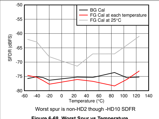
Figure 6-68. Worst Spur vs Temperature
