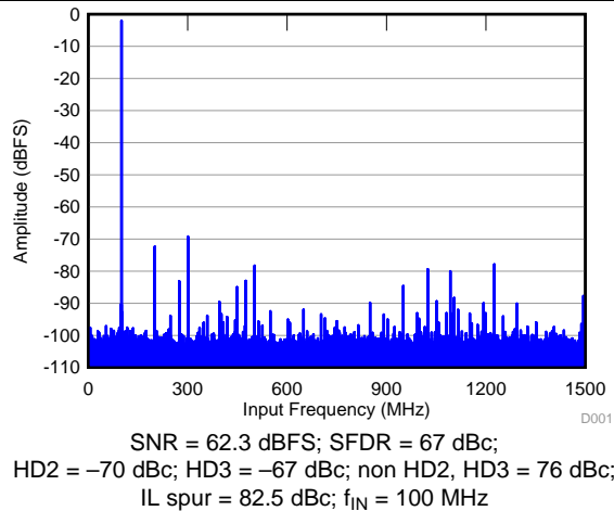
Figure 3. FFT for 100-MHz Input Frequency
