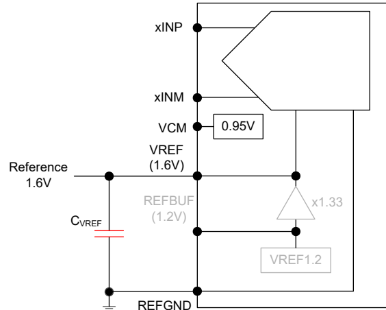
Figure 8-12. External 1.6 V reference
