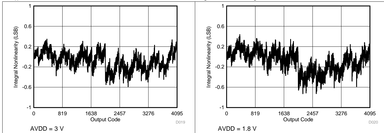
Figure 19. Typical INL in Manual Mode
