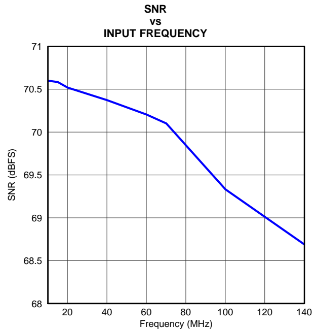
Figure 6-6. SNR vs Input Frequency G006
