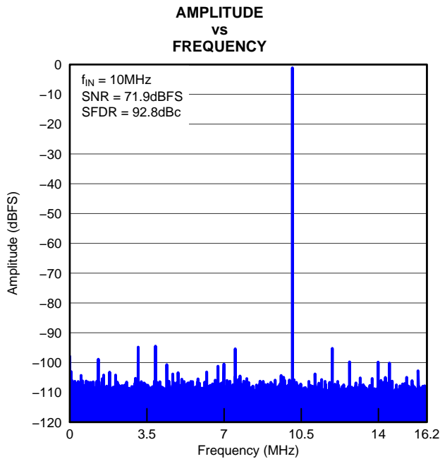
Figure 6-5. Spectrum With Decimation Filter ON G005
