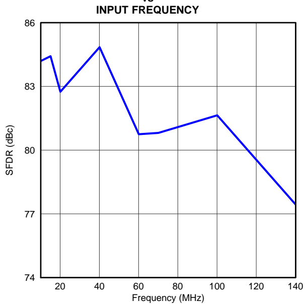
Figure 6-7. SFDR vs Input Frequency G007
