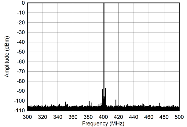
Figure 5-251. Single Tone Spectrum at 400 MHz and -6 dBFS ( \pm 100\text{MHz} )
