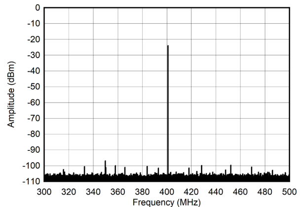
Figure 5-255. Single Tone Spectrum at 400 MHz and -30 dBFS ( \pm 100\text{MHz} )
