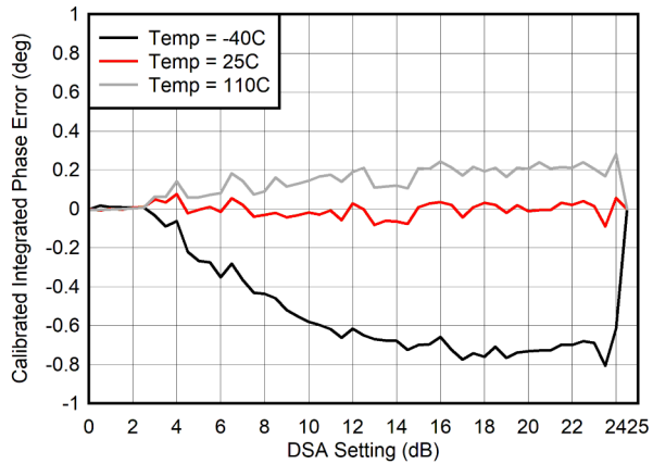
Figure 5-37. RX Calibrated Integrated Phase Error vs DSA Setting at 400 MHz
