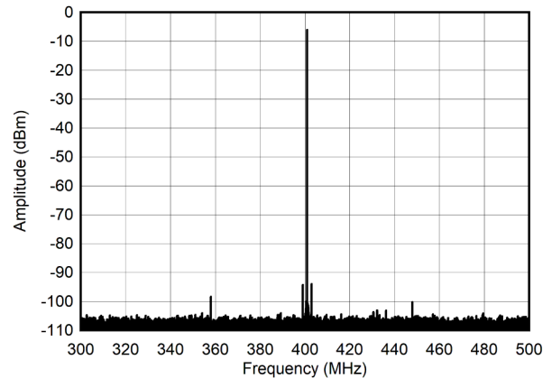
Figure 5-253. Single Tone Spectrum at 400 MHz and -12 dBFS ( \pm 100\text{MHz} )
