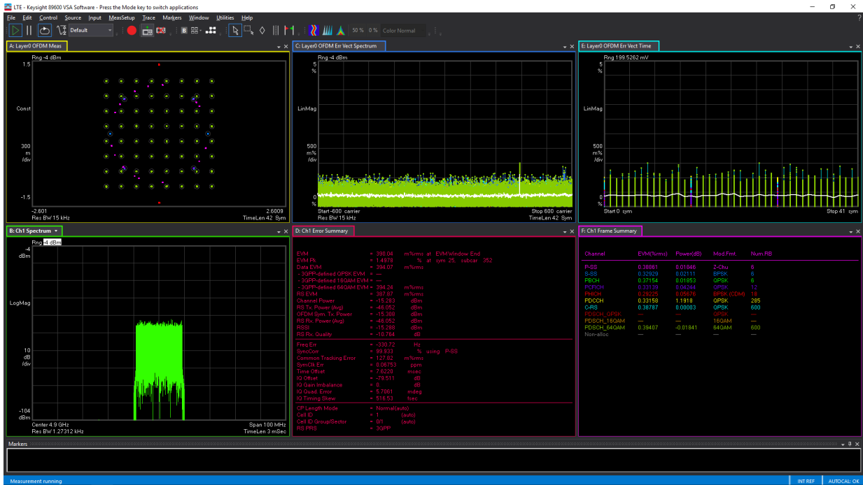
Figure 5-521. TX 20-MHz LTE Error Vector Magnitude at 4.9 GHz
