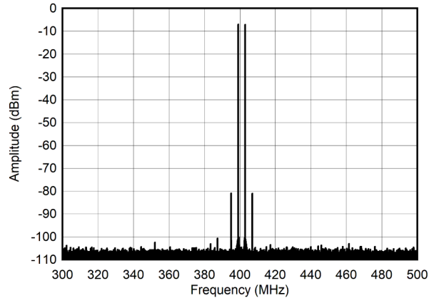
Figure 5-261. Dual Tone Spectrum at 400 MHz and -13 dBFS ( \pm 100\text{MHz} )
