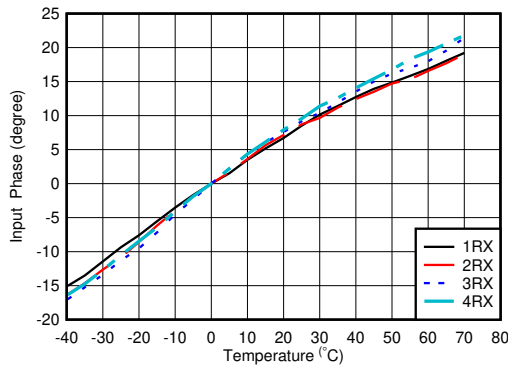
Figure 5-83. RX Input Phase vs Temperature and DSA at f_{IN} = 1.75\text{ GHz}
