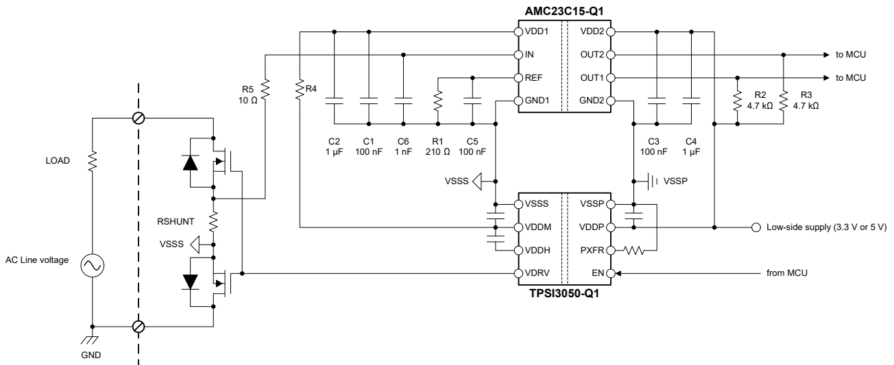
Figure 8-1. Using the AMC23C15-Q1 for Overcurrent and Short-Circuit Detection
