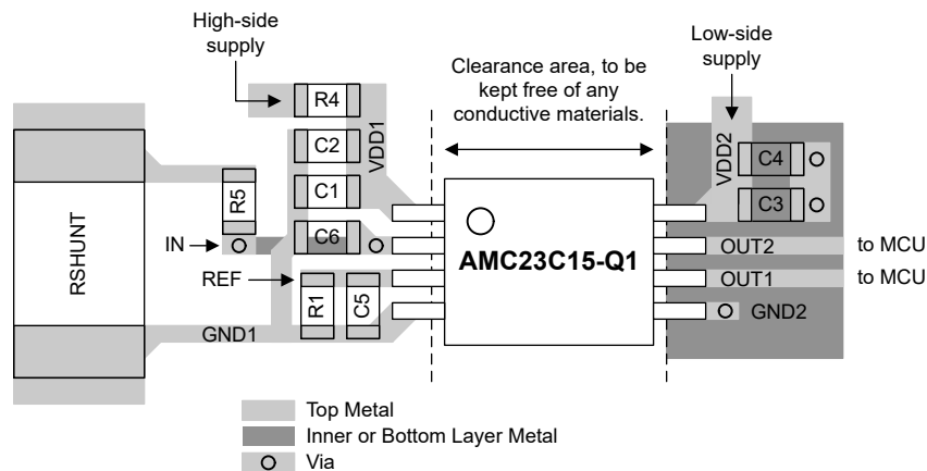
Figure 8-8. Recommended Layout of the AMC23C15-Q1
