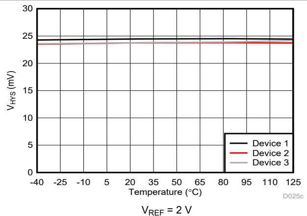
Figure 6-34. Cmp0 Trip Threshold Hysteresis vs Temperature
