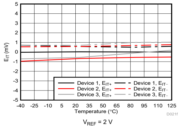
Figure 6-32. Cmp0 Trip Threshold Error vs Temperature
