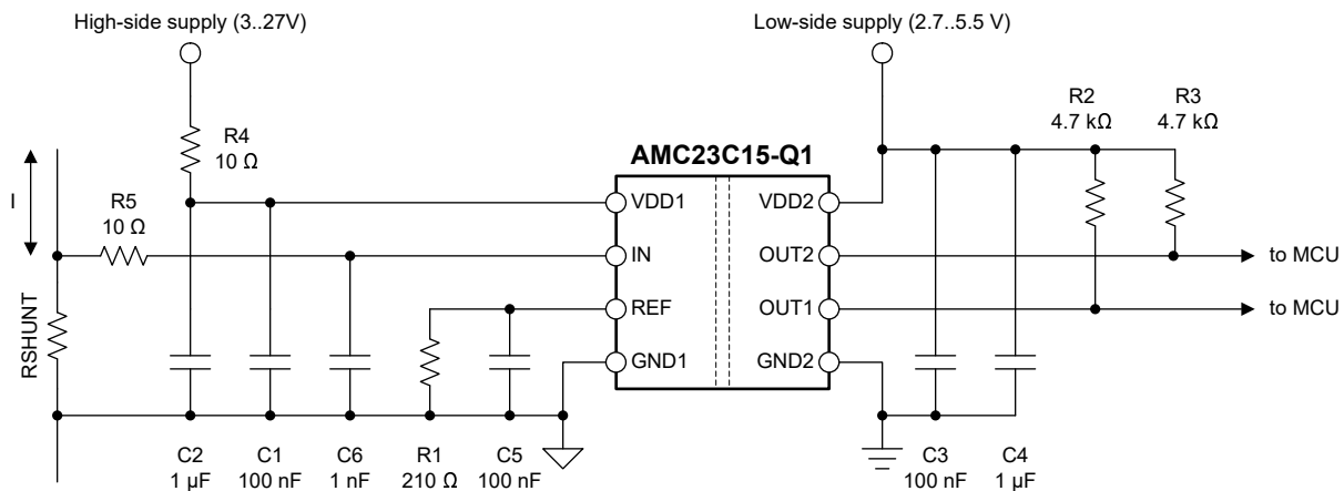
Figure 8-7. Decoupling of the AMC23C15-Q1
