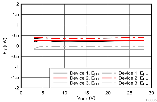
Figure 6-5. Cmp2 Trip Threshold vs Supply Voltage
