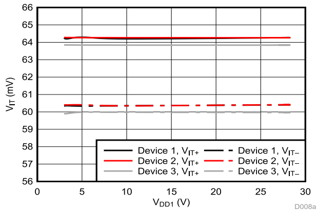
Figure 6-5. Cmp2 Trip Threshold vs Supply Voltage
