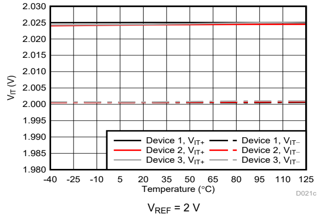
Figure 6-30. Cmp0 Trip Threshold vs Temperature
