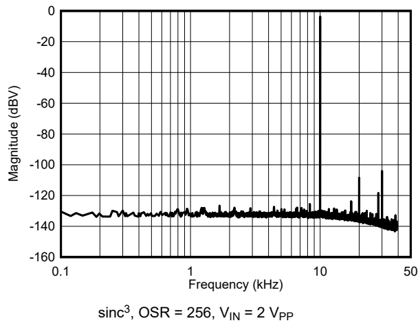
Figure 6-36. Frequency Spectrum With 10-kHz Input Signal
