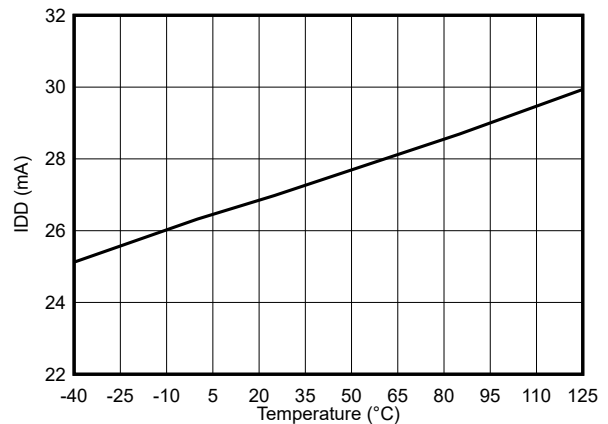
Figure 6-41. Supply Current vs Temperature
