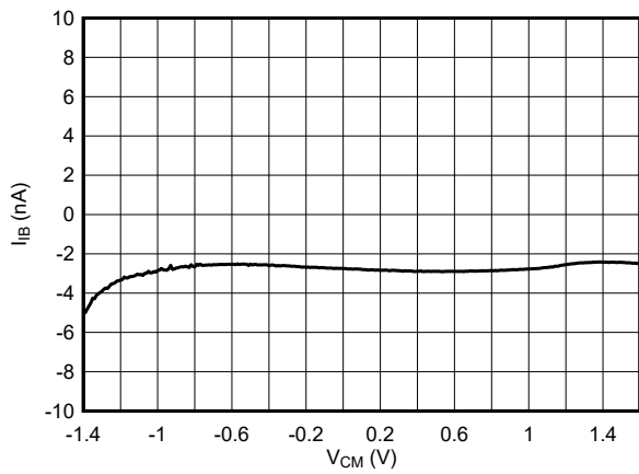
Figure 6-6. Input Bias Current vs Common-Mode Input Voltage
