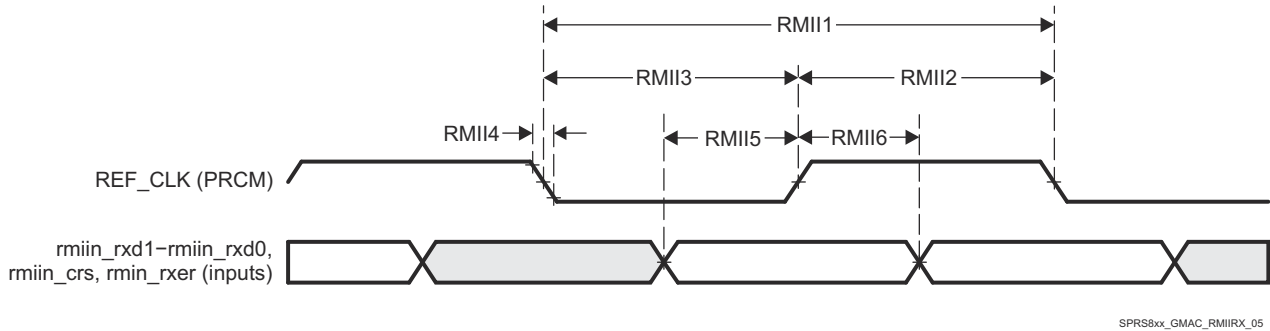
Figure 7-15. MAC Receive Interface Timing, RMIIIn operation
