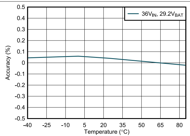
Figure 6-4. Charge Voltage Accuracy vs Temperature
