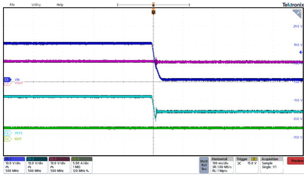
Figure 8-9. VAC to VBAT Power Path Transfer
