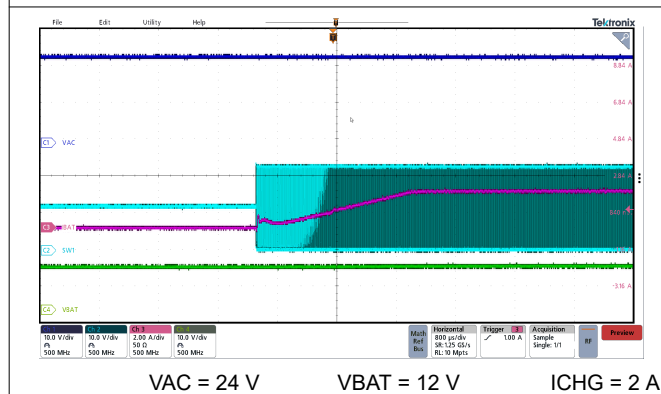
Figure 8-5. Charge Enable via I 2 C with 2-A ICHG
