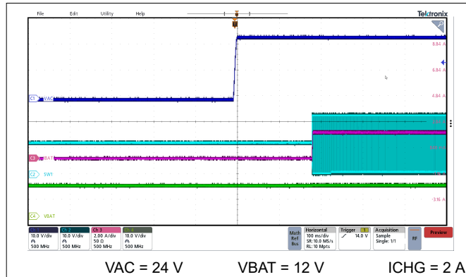
Figure 8-3. VAC Plug-In Power Up with 2-A ICHG
