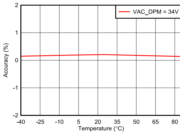
Figure 6-7. Input Voltage ( V_{AC\_DPM} ) Regulation Accuracy vs Temperature
