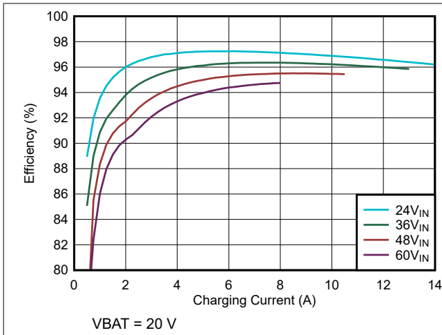
Figure 6-1. Charge Efficiency vs Charge Current (5s battery configuration)
