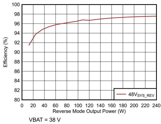
Figure 6-11. Reverse Mode Efficiency (10s battery configuration)
