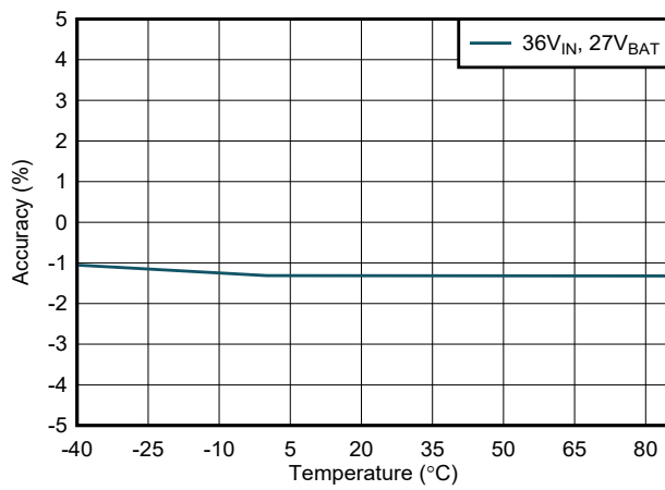
Figure 6-5. Charge Current Accuracy vs Temperature
