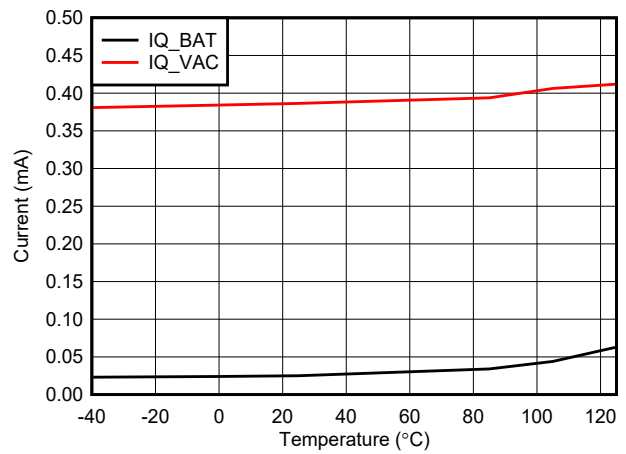
Figure 6-6. Battery and Input Quiescent Current vs Temperature with V_{BAT} = 20 \text{ V}
