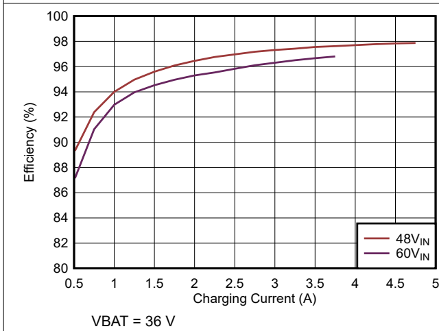
Figure 6-3. Charge Efficiency vs Charge Current (9s battery configuration)
