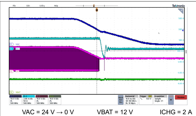
Figure 8-4. VAC Un-plug Power Down with 2-A ICHG
