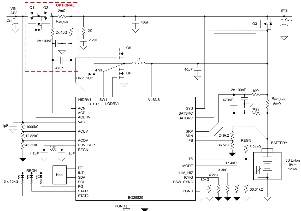
Figure 8-1. BQ25820: I 2 C Controlled, 24 VAC with 3-S Li-Ion Battery, 10-A Charge Current and 350-kHz Switching Frequency
