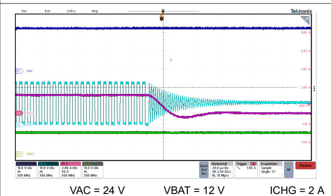
Figure 8-6. Charge Disable via I 2 C with 2-A ICHG
