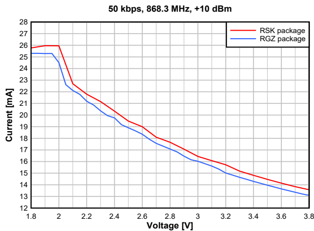
Figure 7-12. TX Current vs. Supply Voltage (VDD5) (50kbps, 868.3MHz)
