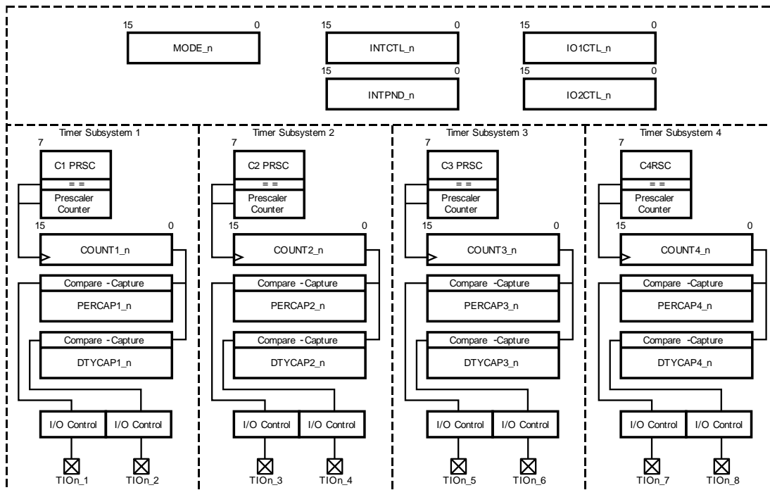
Figure 33-1. Versatile Timer Unit Block Diagram
