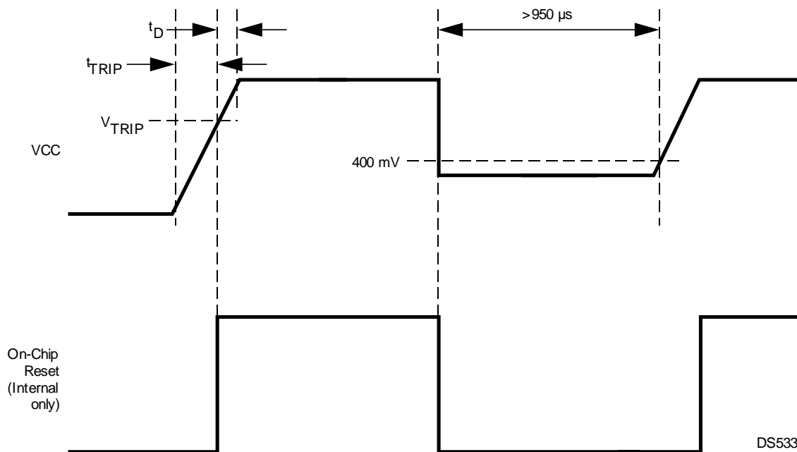
Figure 36-4. Power-On Reset
