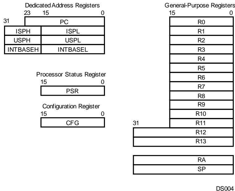
Figure 5-1. CPU Registers
