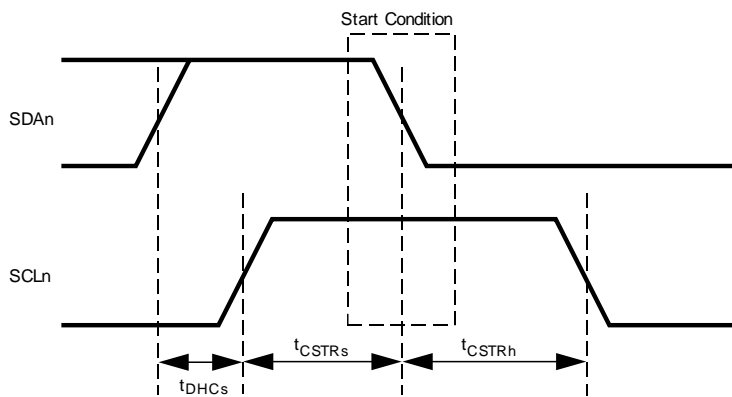
Note: In the timing tables the parameter name is added with an "o" for output signal timing and "i" for input signal timing. DS367
