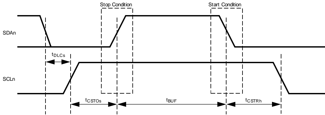
Note: In the timing tables the parameter name is added with an "o" for output signal timing and "i" for input signal timing. DS366
