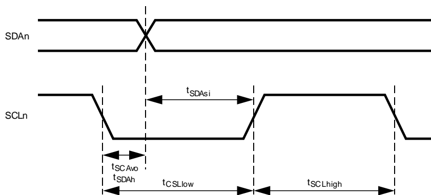
Note: In the timing tables the parameter name is added with an "o" for output signal timing and "i" for input signal timing, unless the parameter already includes the suffix. DS368
