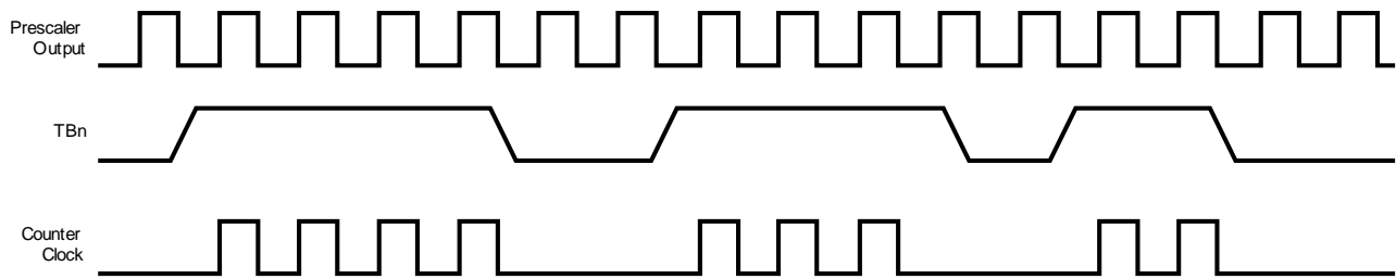
Figure 32-3. Pulse-Accumulate Mode
