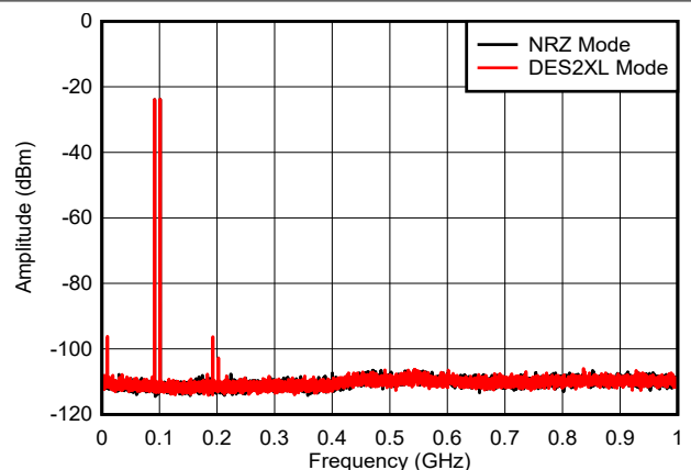
Figure 6-40. Dual Tone, f_{\text{OUT}} = 97\text{MHz} , -6dBFS (0 - 1GHz)
