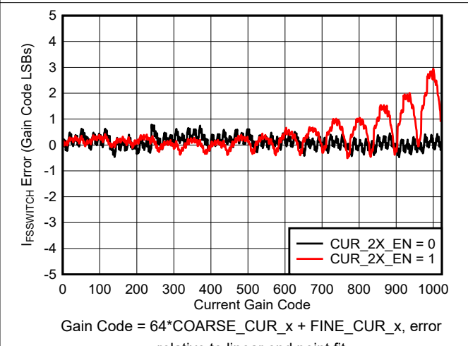
Figure 6-17. I_{\text{FS\_SWITCH}} Error vs Gain Code
