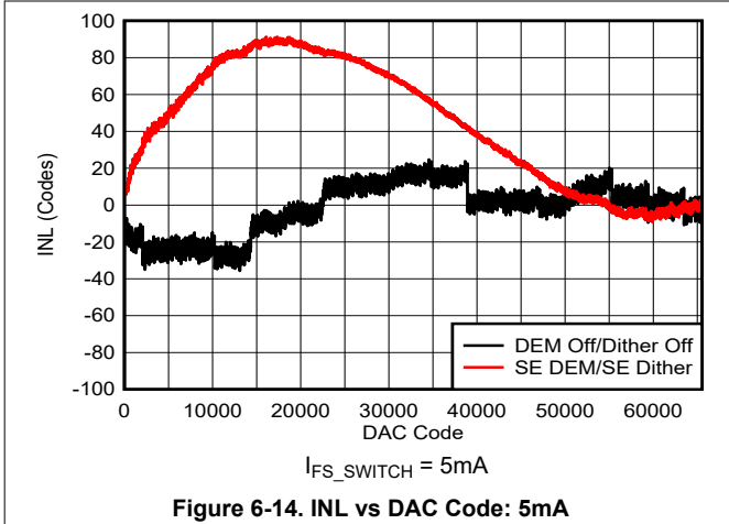
Figure 6-14. INL vs DAC Code: 5mA
