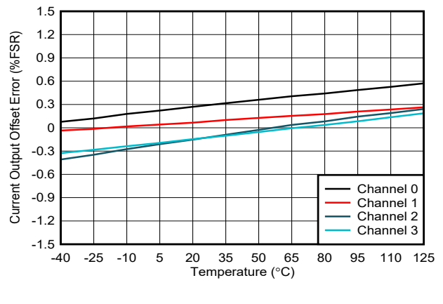
Figure 6-46. Current Output Offset Error vs Temperature
