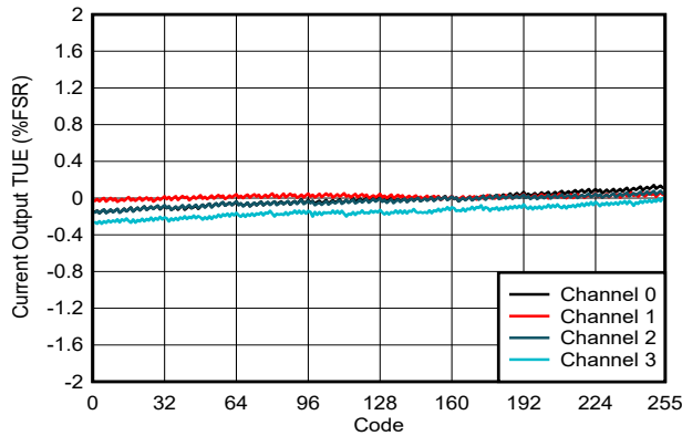
Figure 6-41. Current Output TUE vs Digital Input Code
