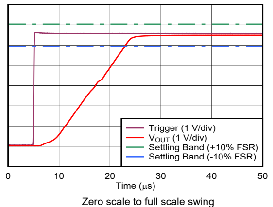
Figure 6-21. Voltage Output Setting Time: Rising Edge
