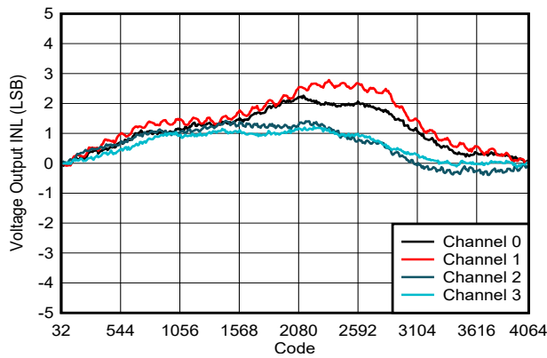
Internal reference, gain = 4 × Figure 6-4. Voltage Output INL vs Digital Input Code
