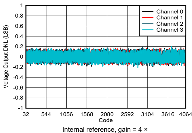
Internal reference, gain = 4 × Figure 6-8. Voltage Output DNL vs Digital Input Code
