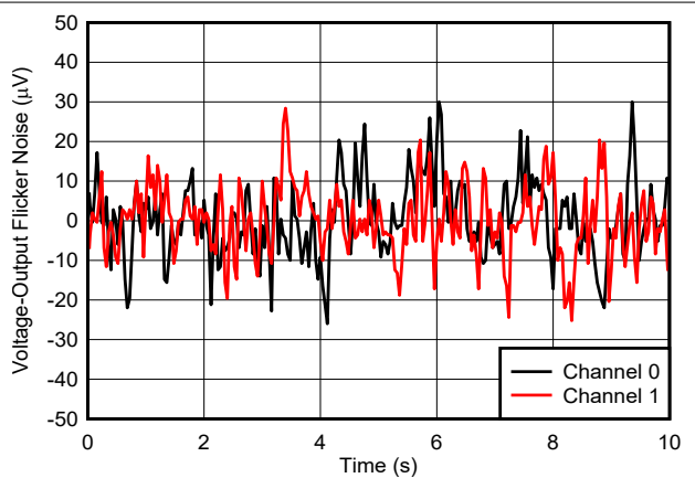
Figure 5-27. Voltage Output Flicker Noise
