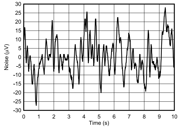
Figure 7-47. DAC Output Noise: 0.1 Hz to 10 Hz
