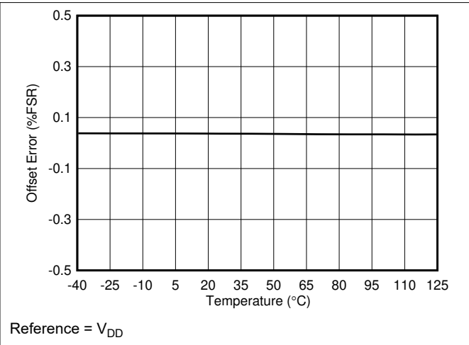
Figure 7-9. Offset Error vs Temperature
