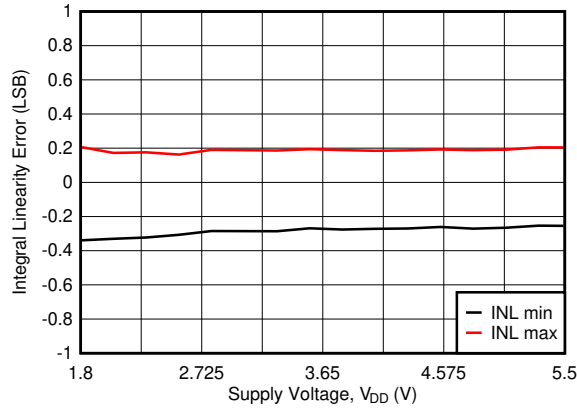
Figure 7-22. Integral Linearity Error vs Supply Voltage
