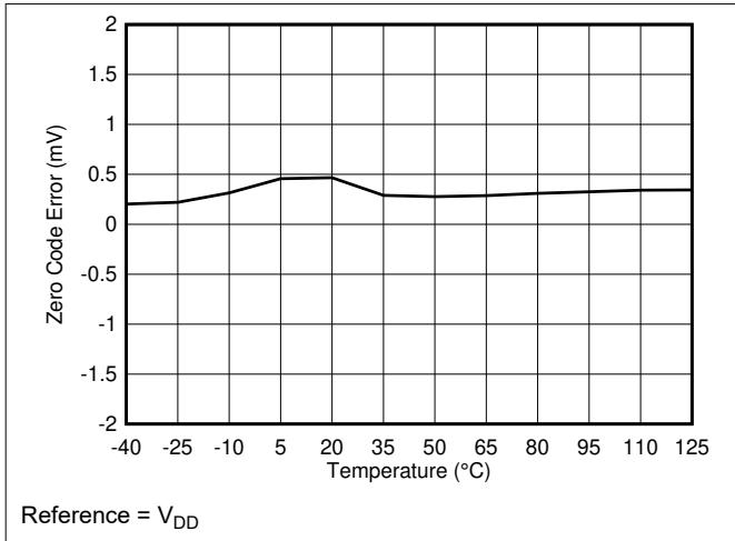
Figure 7-8. Zero Code Error vs Temperature
