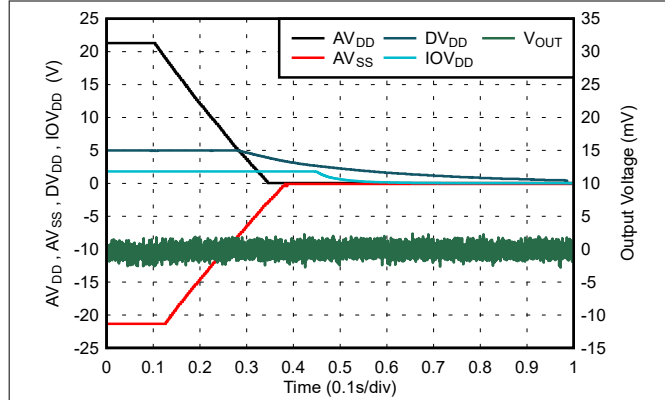
Figure 5-40. Power-Down Response
