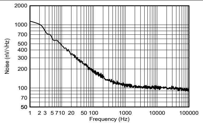
Figure 5-41. DAC Output Noise Density vs Frequency
