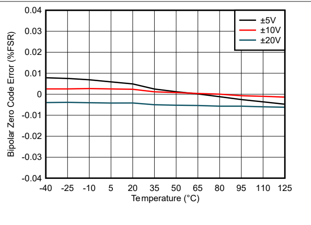
Figure 5-23. Bipolar Zero Code Error vs Temperature
