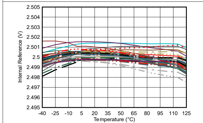
Figure 5-44. Internal Reference Voltage vs Temperature (TSSOP)
