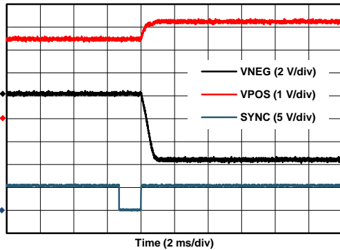
Figure 83. Buck-Boost Converter Power-On (IOOUT Mode)
