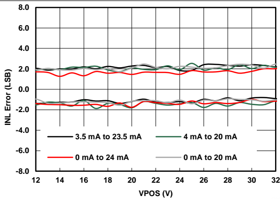
Figure 15. IOU Linearity Error vs Power Supplies
